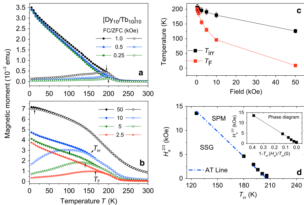
Fig. 1 Field cooled (FC) and zero field cooled (ZFC) measurements. a, b The plot of in-plane magnetization versus temperature for the [\text{Dy}_{10}/\text{Tb}_{10}]_{10} sample. The measurements were done on heating at various fields (indicated in the figure) after ZFC and FC in 70 kOe (7000 mT). A broad maximum can be observed for the ZFC curves ( T_F ) followed by a furcation point ( T_{irr} ) with the FC curves. Presence of a maximum for the ZFC curves at fields of 10 kOe (1000 mT) and lower indicates a freezing-like state. c The plot of T_{irr} and T_F as estimated from the ZFC and FC curves versus increasing fields of measurement H_a . The lines are guide to the eye. Error bars represent standard error of the measured temperature value. d The plot of H_a^{2/3} versus T_{irr} showing T_{irr}(0) = 205 K. The blue line is the linear fit to the data following the Almeida-Thouless (AT) equation. The inset of (d) shows phase diagram of the same in a plot of H_a^{2/3} as a function of 1 - T_{irr}(H_a)/T_{irr}(0) . The region below the line is SSG while it is SPM above
