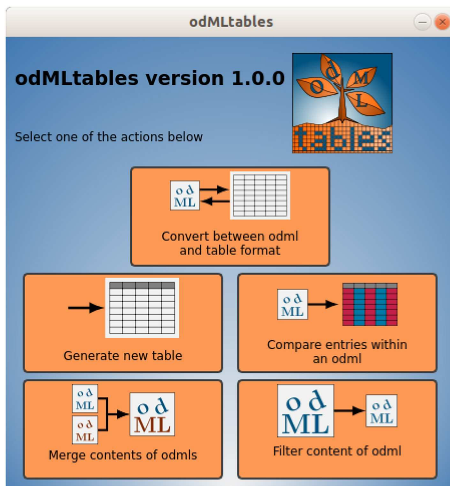
FIGURE 5 | Main window of the odMLtables GUI. The interface gives access to the main functionalities available by the tool: converting files from hierarchical to tabular (flat) representations, generating an empty generic odML table (template), comparing entries within a metadata collection, merging contents of two collections, and selecting a subset of a metadata collection (filtering). Each button starts a series of dialogs (wizards) that guide the user through the corresponding process.
