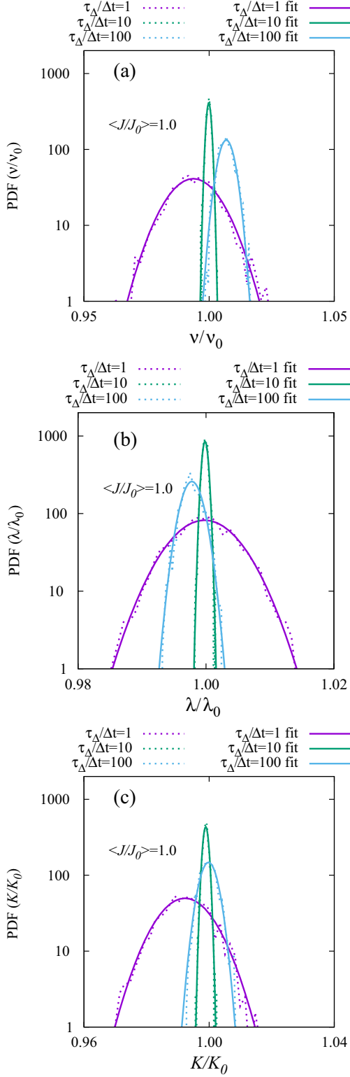
FIG. 7. Shown are the distribution functions (a) PDF( v/v_0 ), (b) PDF( \lambda/\lambda_0 ), and (c) PDF( K/K_0 ) for the reconstruction using different increments \tau_\Delta/\Delta t = 1, 10, 100 and based on 200 snapshots of the simulation with \langle J/J_0 \rangle = 1 . Gaussian fits G(v/v_0) , G(\lambda/\lambda_0) , and G(K/K_0) are also shown in the figure based on moments of v , \lambda , and K computed for the series of reconstruction results. The narrowest distribution occurs in all cases (a), (b) and (c) for the parameter \tau_\Delta/\Delta t = 10 , the widest for \tau_\Delta/\Delta t = 1 .
