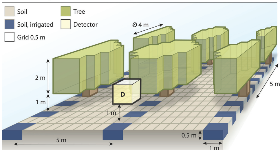
Schematic segment of the URANOS setup , total extent: 500 m
