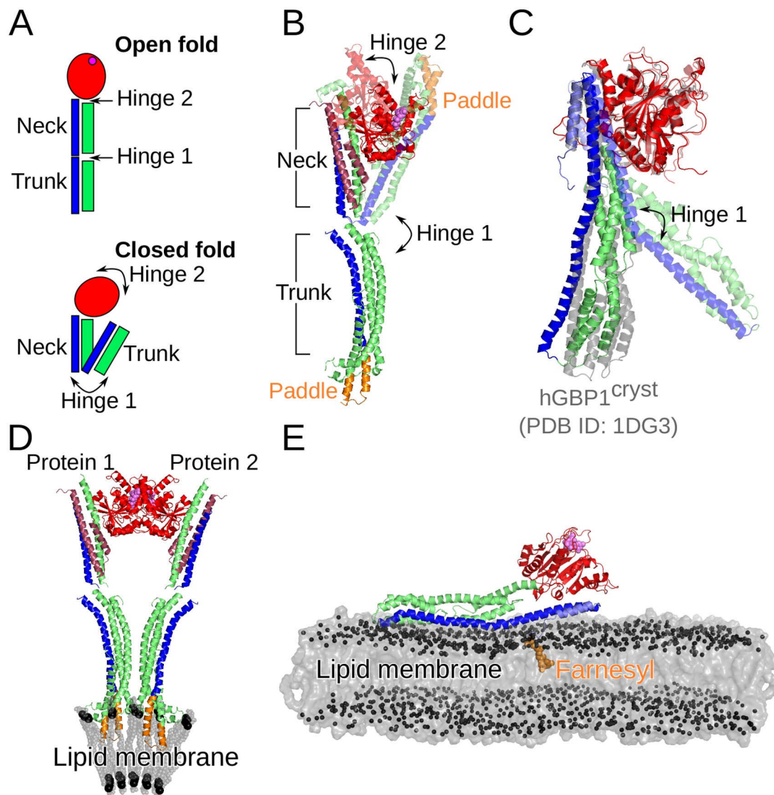
Fig 8. Conformational transitions of hGBP1 and a bacterial dynamin-like protein (BDLP) of Nostoc punctiforme . (A) Schematic providing nomenclature for the open and closed BDLP conformations with large-scale transitions between them mediated by hinges 1 and 2 at the trunk/neck and neck/G-domain interfaces. As for hGBP1, the GTPase domain is colored in red with the position of the nucleotide in the open conformation indicated by a magenta sphere, while the 4-helix bundle composing the neck and trunk is colored in green and blue. (B) The closed conformation of BDLP was solved by X-ray crystallography (PDB 2J69, shown in transparent cartoon), while the open conformation was determined by cryo-electron microscopy (PDB 2W6D, shown in opaque cartoon). The two helices preceding the G domain are ruby-colored. (C) From our MD simulations of hGBP1 we observed a kinking of the M and E domain resembling the initial stages of the closed \leftrightarrow open transition of BDLP around hinge1, as the overlay of the structures representing this motion (i.e., FEM1 and PC1 min in Fig 4) shows. For comparison the crystal structure of hGBP1 (PDB 1DG3) is also shown (in gray). (D) Membrane binding of BDLP occurs following nucleotide binding via the paddle domain (shown in orange) in the open conformation and aggregated BDLP state. Aggregation involves association of the G domains. (E) Membrane binding of hGBP1 also requires nucleotide binding and is facilitated via farnesylation (shown in orange) at the C-terminus acting as lipid anchor.
