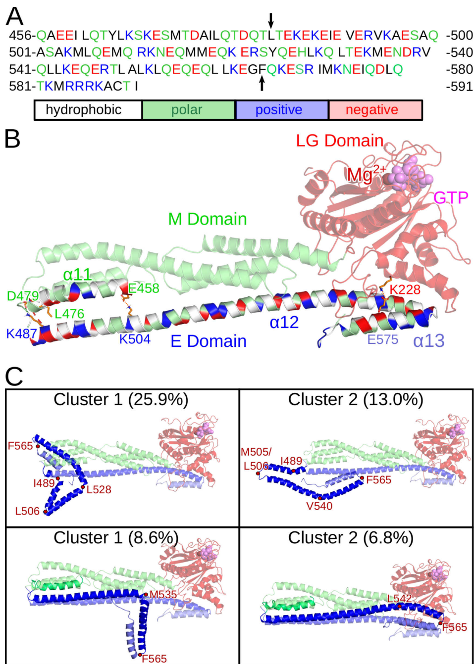
Fig 5. Properties and dynamics of the isolated E domain of hGBP1. (A) The sequence of the E domain and preceding helix \alpha 11 of the M domain is shown and colored according to the physicochemical properties of the amino acids. The start and end of helix \alpha 12 at residues L482 and F565 are indicated by vertical arrows. (B) The structure of the E domain and its interactions with the LG domain (red transparent) and the helix \alpha 11 of the M domain (green transparent) are highlighted for the crystal structure of hGBP1 (PDB 1DG3). The residues of \alpha 11 and the E domain are colored according to the physicochemical properties of the amino acids: white, hydrophobic; green, polar; blue, positively charged; red, negatively charged. Salt bridges (K228–E575, E458–K504, D479–K487) are indicated with orange dashes and hydrogen bonds (L476/D479–K487) with black dashes. The interacting residues are shown as sticks and labeled. This includes K582 and K587, which form salt bridges with various residues of loop L1 (in yellow) of the LG domain. (C) The two most populated cluster conformations with their occurrence obtained from the MD simulations of the isolated E domain (top) and of \alpha 11 plus E domain (bottom). The cluster structures were aligned to the crystal structure of full-length hGBP1 (shown as transparent cartoon) using residues 482–484 for the alignment of the isolated E domain and \alpha 11 for alignment of \alpha 11 plus E domain. The red points indicate the turns that formed at the different positions of the E domain along with the turn at F565 separating \alpha 12 and \alpha 13 from each other.
