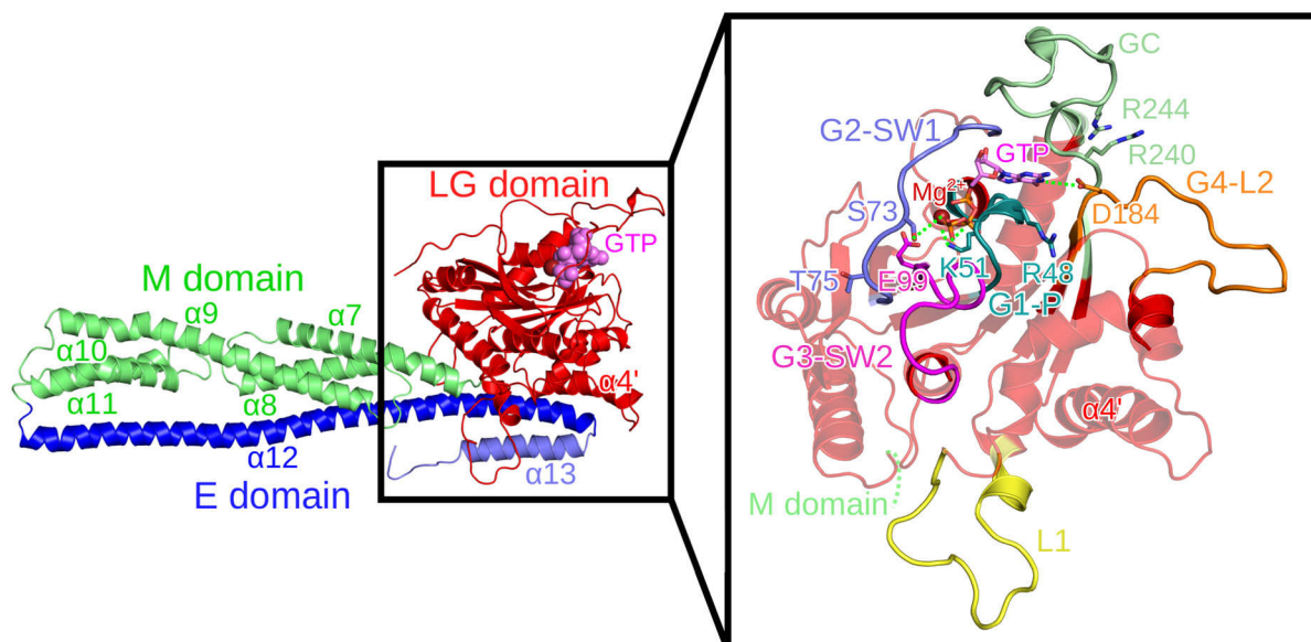
Fig 1. Conformation of the nucleotide-bound hGBP1 crystal structure (PDB 1F5N). The different domains are highlighted in different colors: the LG domain in red with GTP shown in purple, the M domain in green, and the E domain in blue (with different shades used for \alpha 12 and \alpha 13 for ease of distinction). Loops missing in the crystal structure were modeled. In the enlargement of the LG domain shown on the right, the four GTP-binding site motifs are displayed: the G1-P loop in turquoise, G2-SW1 in blue, G3-SW2 in magenta, and G4-L2 in orange. The guanidine cap (green), loop L1 (yellow), and residues important for dimerization or GTP binding and hydrolysis (shown as sticks with the same color as the corresponding loop) are also highlighted. The dotted green lines indicate direct interactions of hGBP1 residues with GTP and Mg^{2+} .
