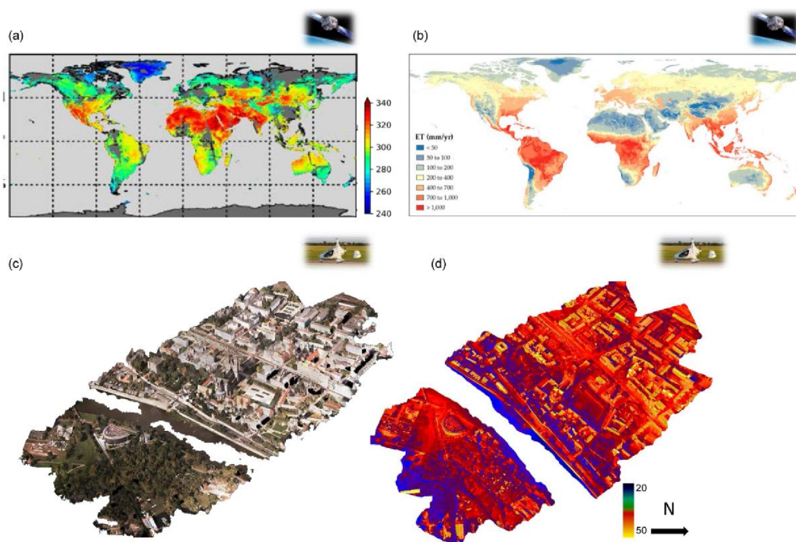
Figure 11. Land surface temperature and related traits: (a) Daytime land surface temperature (LTS) composite. Derived from Aqua MODIS RS data for 1 June 2010 (from Ghent et al. [385]), (b) daily global evapotranspiration using Menman–Ponteith equation and remotely sensed land surface temperature (Raouf and Beighley, [386]). (c) Near 3D-True-Ortho-RGB image of Magdeburg (City Centre) RGB image, (d) 3D-TIR image based on the Aerial Oblique System [AOS-Tx8] with 8 cameras (4 cameras FLIR A65 SC, 4 RGB cameras Baumer VC XG-53c) rendered as a 3D TIR image of Magdeburg. (c,d) were taken by Prof. Lutz Bannehr, Department of Architecture, Facility Management and Geoinformation, Institute for Geoinformation and Surveying, Dessau, Germany.
