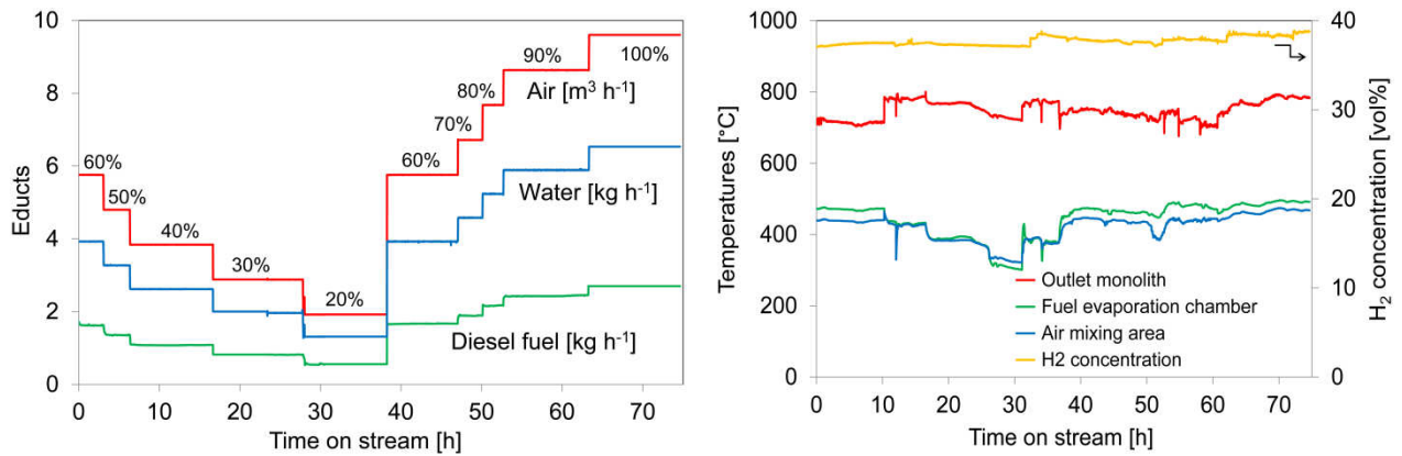
Figure 2 Left: Mass streams and volumetric flow of the educts during a load change experiment using the pulse valve for diesel fuel injection, n(\text{O}_2)/n(\text{C}) = 0.47 , n(\text{H}_2\text{O})/n(\text{C}) = 1.9 , \text{TAI} = 380\text{ }^\circ\text{C} , \text{TCB} = 230\text{ }^\circ\text{C} , Ultimate diesel fuel, mass fraction of cold water to the nozzle: 40% Right: Temperatures inside the ATR and dry H 2 concentrations in the reformat during a load change experiment using the pulse valve for diesel fuel injection, n(\text{O}_2)/n(\text{C}) = 0.47 , n(\text{H}_2\text{O})/n(\text{C}) = 1.9 , \text{TAI} = 380\text{ }^\circ\text{C} , \text{TCB} = 230\text{ }^\circ\text{C} , Ultimate diesel fuel, mass fraction of cold water to the nozzle: 40%
