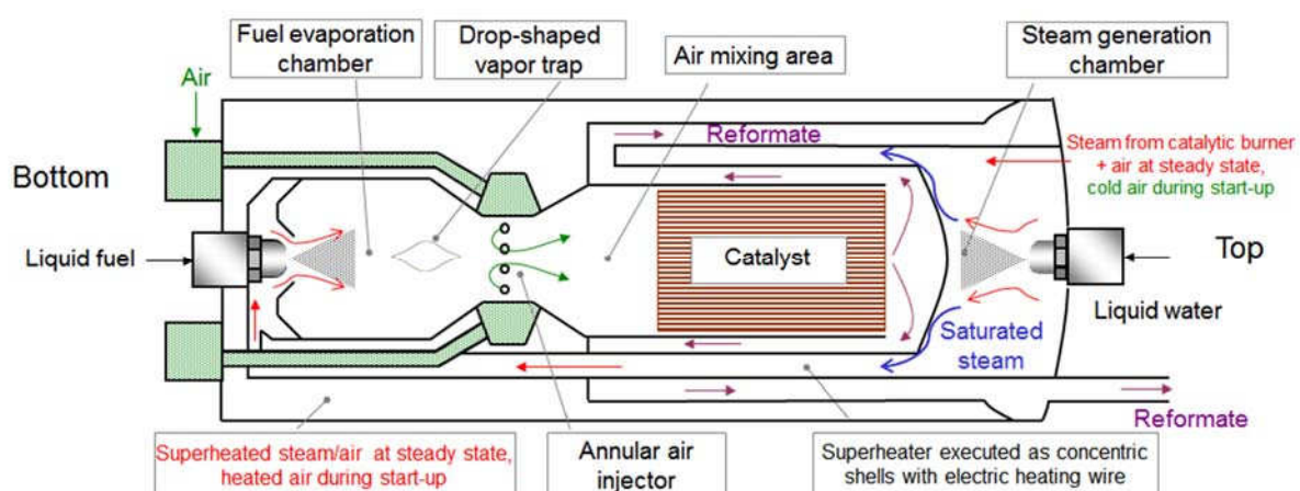
Figure 1 Design of Jülich's autothermal reformer, ATR 14
