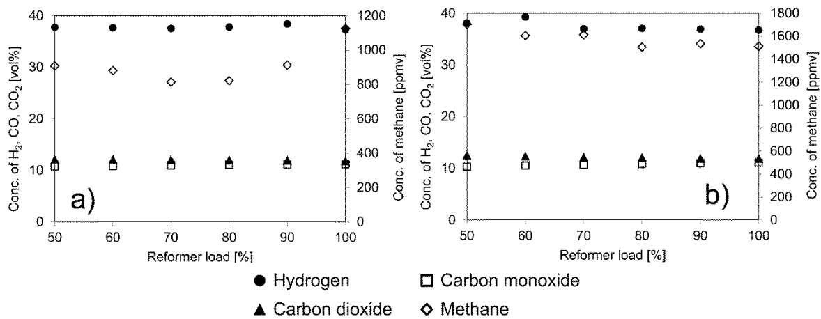
Figure 4 Dry concentrations of the main products of ATR 14 as a function of the reformer load, n(\text{O}_2)/n(\text{C}) = 0.47 , n(\text{H}_2\text{O})/n(\text{C}) = 1.9 , \text{TAI} = 380\text{ }^\circ\text{C} , \text{TCB} = 230\text{ }^\circ\text{C} , Fuel: Ultimate diesel, mass fraction of cold water to the nozzle a) = 30%; b) = 40%
