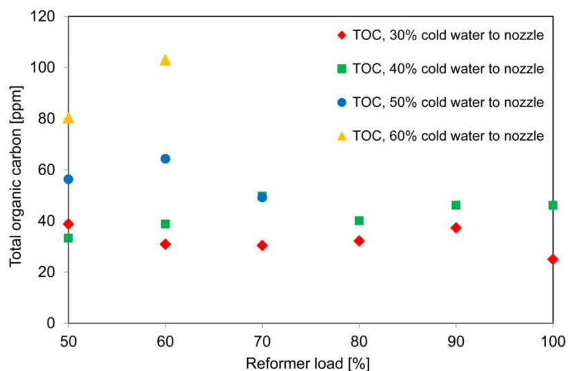
Figure 7 Total organic carbon (TOC) in the condensed water as a function of the reformer load at different mass fractions of cold water to the nozzle, n(\text{O}_2)/n(\text{C}) = 0.47 , n(\text{H}_2\text{O})/n(\text{C}) = 1.9 , \text{TAI} = 380\text{ }^\circ\text{C} , \text{TCB} = 230\text{ }^\circ\text{C} , fuel: Ultimate diesel
