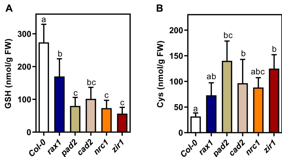
Fig 1. Glutathione content in a series of allelic mutants deficient in glutamate-cysteine ligase. (A,B) HPLC analysis of total glutathione presented as GSH equivalents (A) and cysteine (B) in 5-day-old seedlings. The presented values are means \pm SD ( n = 5 ). Lower case letters indicate statistically different values (One-way ANOVA with Tukey's multiple comparisons test; p < 0.05 ).
