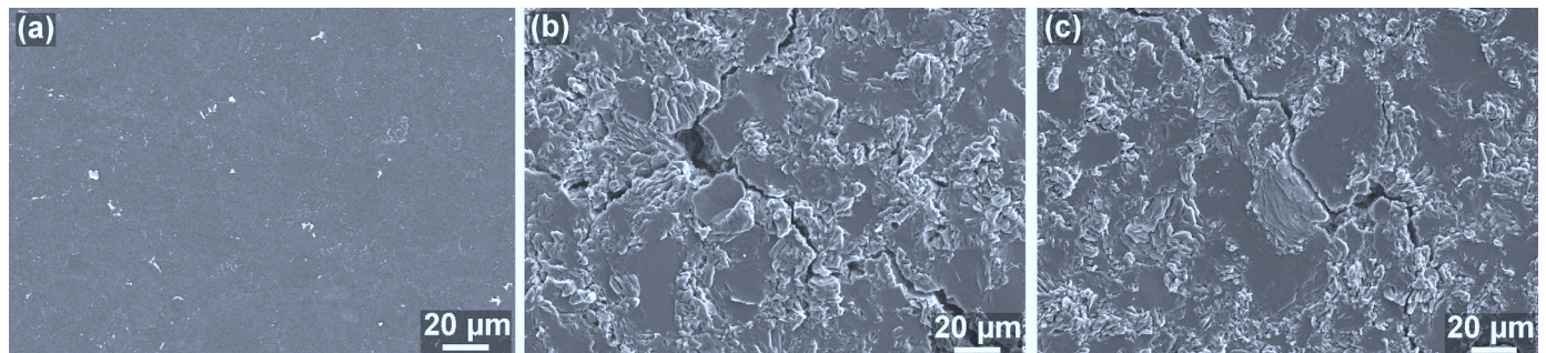
Fig. 3. Scanning electron microscopy images of S-65 beryllium samples loaded in JUDITH 1 (a) and JUDITH 2 (b), (c) with F_{\text{HF}} = 3 \text{ MW m}^{-2} \text{ s}^{0.5} at T_{\text{base}} = 523 \text{ K} with different numbers of pulses. (a) 10^3 pulses, no visible damage. (b) 10^5 pulses, small cracks. (c) 10^6 pulses, small cracks.
