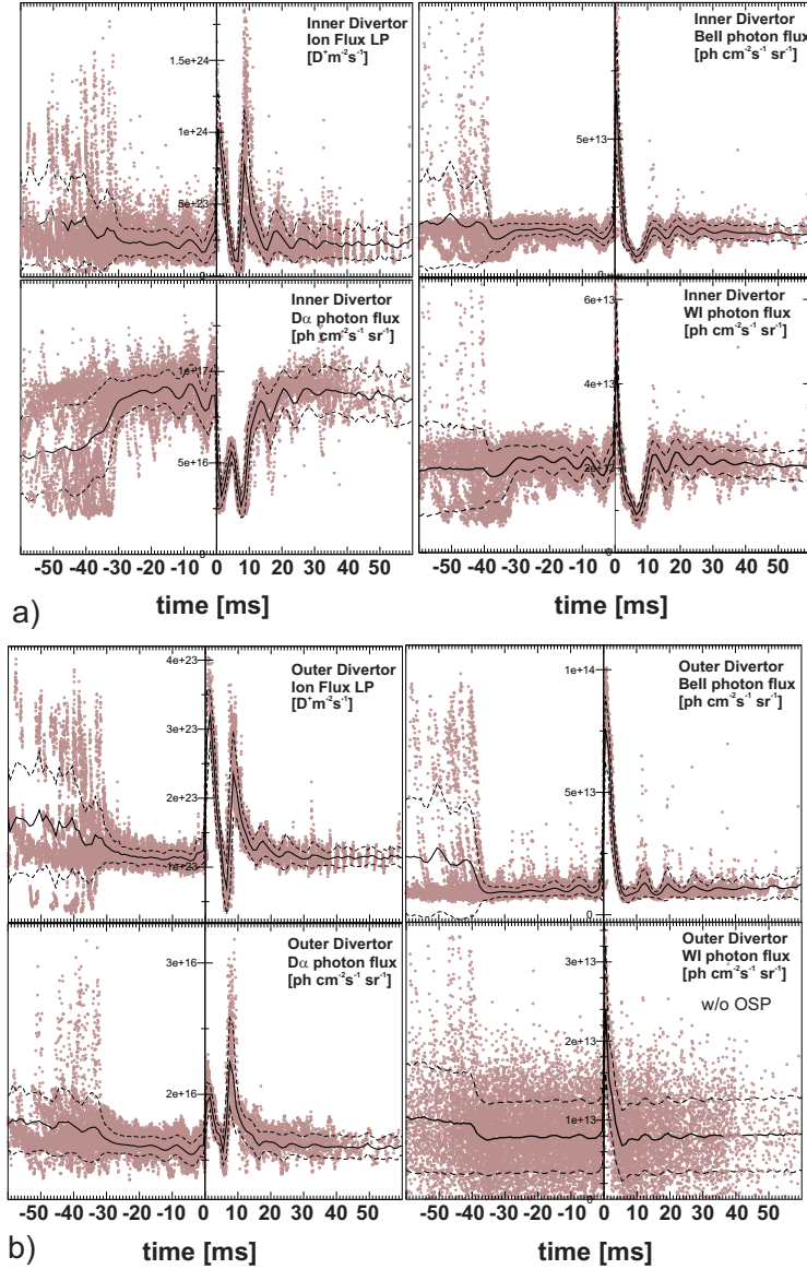
FIG. 11: a) ELM averaging at the inner divertor leg: impinging deuteron flux density (Langmuir probes), recycling flux density ( D_\alpha ), Be impurity flux ( BeII at \lambda = 527.0nm ), gross W sputtering flux density ( WI at \lambda = 400.9nm ). b) Corresponding ELM averaging at the outer divertor leg [w/o OSP].
