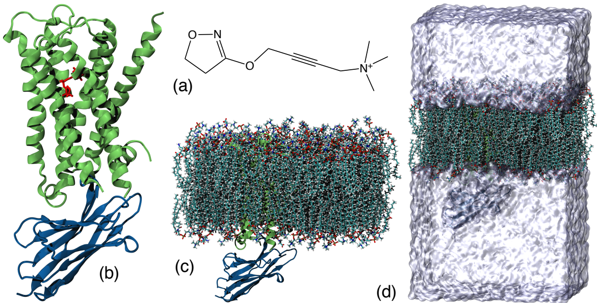
Figure 1: The human M_2 receptor in complex with its agonist iperoxo. (a): The ligand (4-(4,5-dihydro-1,2-oxazol-3-yloxy)but-2-ynyl-trimethylazanium) in 2D representation. (b): M_2 receptor (green) and its bound ligand, along with the Nb 39 nanobody (blue). (c): neuronal membrane with the receptor embedded in it. (d): the simulated system ( \sim 150,000 atoms), formed by ligand, receptor, membrane, water and ions (the latter represented with a transparent surface for sake of clarity).
