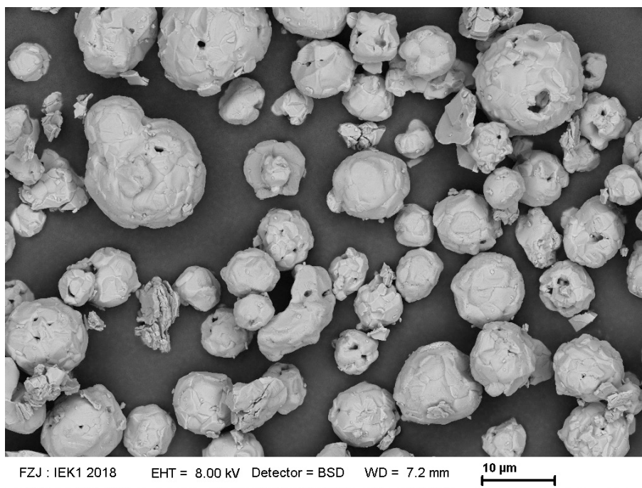
Figure 1. LaWO feedstock powder (SEM back scattered electron image).
