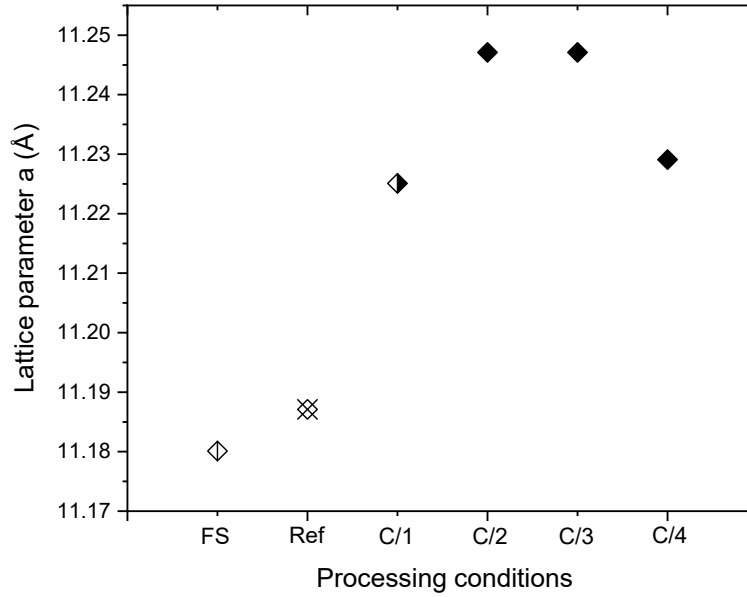
Figure 7. Lattice constant of the main LaWO cubic phase as function of the processing conditions. FS: feedstock; Ref: [12]; C/1: graphite supported coating; C/2-C/4: Crofer supported coatings.
