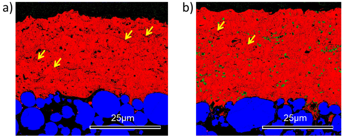
Figure 8. EBSD micrographs showing phase distributions of the main cubic LaWO phase (red) and the secondary phases La 2 O 3 (pointed by yellow arrows) and La 6 W 2 O 15 (green) in a) sample C/6 coated with extra O 2 and annealed in Ar and b) in sample C/7 coated with extra O 2 and annealed in air; the coating contains mainly the cubic LaWO phase (red), while the secondary phases La 2 O 3 (yellow) and La 6 W 2 O 15 (green) are in negligible amounts; La 6 W 2 O 15 is more likely to be found surrounding pores after contact with air.
