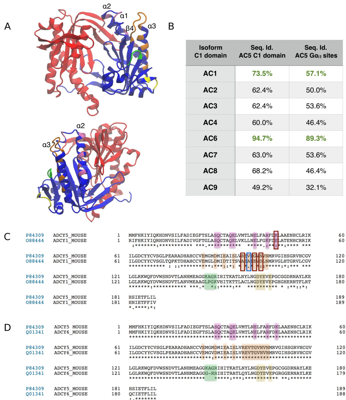
Fig 5. A The structure of the C1 (blue and highlight colors) and C2 (red) catalytic domains of AC5. B The highlighted regions show the AC5 residues that interact with Gα i during complex formation. Overall sequence similarity for the C1 domain for the other mouse AC isoforms, compared to mouse AC5, and for the highlighted residues that interact with Gα i . C, D Pairwise sequence alignments for AC1 (C) and AC6 (D) with the colors matching those of the structure in subfigure A. The mouse sequences were taken from Uniprot, and aligned using Clustal Omega within Uniprot. The C1 domain was identified through alignment with PDB 1CJK [22], which contains a canine AC5 C1 domain, and the residues are numbered from the start of the C1 domain. The first residues of the C1 domains are at positions 288, 456 and 363 in the canonical sequences of AC1, AC5 and AC6 respectively. The red boxes in (C) indicate charge-altering substitutions between the AC5 and AC1 sequences in the Gα i binding α3 helix, while the blue box indicates a substitution in a residue whose mutation was found to affect Gα i -induced inhibition of AC5 [21].
