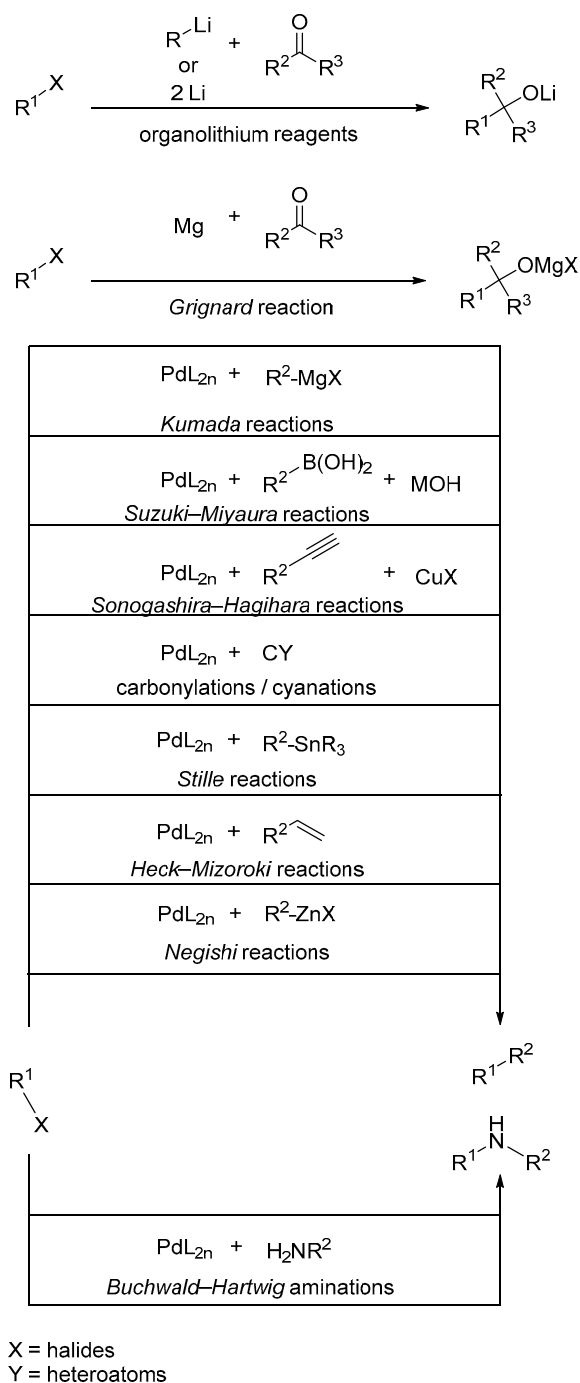
Figure 4. Most common reactions in organic synthesis exploiting halogen moieties. [37,45–48] Besides organolithium reactions as well as Grignard/Barbier reactions all of them are Pd-based, but can in many cases be substituted by other transition metals such as nickel.
