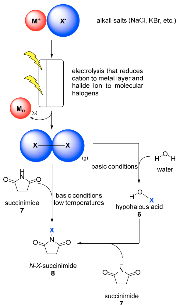
Figure 3. Workflow for the provision of halogenating reagents from alkali salts. The electrolysis process thus produces molecular halogens ( X_2 ), as well as hypohalous acids ( HOX , 6) and N -halogenated succinimides ( NXS , 8) in further steps.
