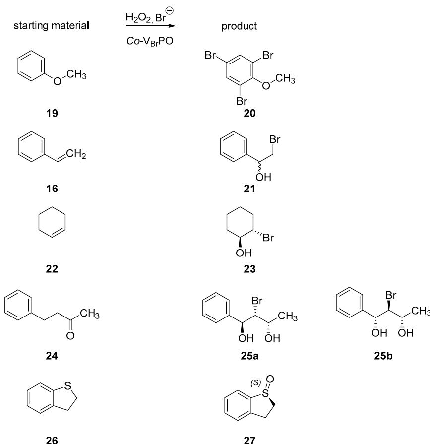
Figure 11. Selected reactions performed by the Co-V Br PO to illustrate the reaction spectrum [81].
