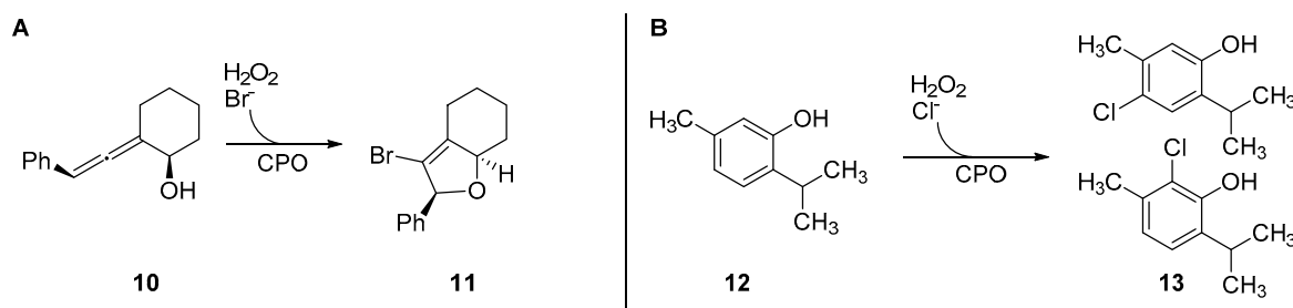
Figure 8. Example reactions of Cf -CPO involved in biocatalytic conversions of organic molecules (A): Cyclization of allenol ( 10 ) to the product 11 induced by halogenation with \text{Br}^- by Cf -CPO. (B): Unselective chlorination of thymol ( 12 ) by Cf -CPO.
