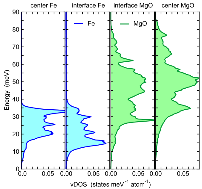
FIG. 9. Layer-resolved vibrational density of states of \text{Fe}_8/(\text{MgO})_8(001) obtained from DFT calculations. Colors and symbols as in Fig. 3. Again, we show only the central layers of the slabs (leftmost panel for Fe and rightmost for MgO) and the interface layers (middle). The entire vDOS including the four intermediate layers is provided in the Supplemental Material [25].
