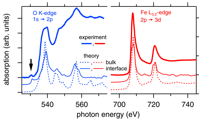
FIG. 2. High resolution x-ray absorption spectra of [\text{Fe/MgO}]_4 with 2 nm individual layer thickness measured in transmission geometry (thick lines), normalized to the incident x-ray intensity. The Fe spectrum (red, at right) is composed of the L_3 and L_2 edges at 708 and 722 eV, respectively. The spectrum at the O K edge (blue, at left) contains several features in agreement with literature [27–29] and the vertical arrow points at the pre-edge feature assigned to an interface state, see text. Calculated atomic-layer-resolved spectra of \text{Fe}_8/(\text{MgO})_8 are shown by thin lines. Spectra at the interface are shown by a solid line, those from the center of the respective layers are shown by a dashed line. Spectra are shifted vertically for better visibility.
