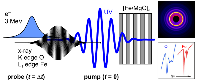
FIG. 1. Schematic of UV pump, electron diffraction, and soft x-ray absorption probe experiment. In both cases, the signal transmitted through the [\text{Fe}/\text{MgO}]_n heterostructure was detected. At right, exemplary data are shown: Electron diffraction image in transmission with the diffraction intensity represented in a false color scheme (top) and x-ray transmission spectra (bottom) for the O K edge including a pre-edge feature originating from the Fe-MgO interface (blue) and the Fe L_3 edges (red).
