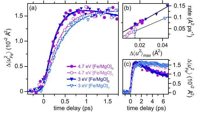
FIG. 8. (a) Change of the r.m.s. displacement \Delta\langle u^2 \rangle(t) as a function of pump-probe time delay for the different sample configurations ( [\text{2 nm Fe}/5 \text{ nm MgO}]_5 —filled symbols; [\text{10 nm Fe}/25 \text{ nm MgO}]_1 —open symbols) and excitation conditions (pump photon energy 4.7 eV—circles, 3.1 eV—triangles); the solid and dashed curves represent fits to the measured data as explained in the text. (b) Maximum rate of the increase of \Delta\langle u^2 \rangle(t) obtained from the fits as shown in panel (a) for a range of pump fluences. The different values of maximum \Delta\langle u^2 \rangle were obtained from pump fluences ranging from 6 to 15 \text{mJ}/\text{cm}^2 . Photon energies are indicated by symbols, see panel (a). Solid curves: Linear guide to the eye. (c) \Delta\langle u^2 \rangle(t) over a larger delay time range.
