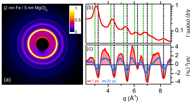
FIG. 6. (a) Electron diffraction pattern of a [2 nm Fe/5 nm MgO] 5 heterostructure in false color representation. (b) Scattering intensity I(q) as a function of momentum transfer q of this heterostructure. (c) Difference scattering pattern \Delta I(q, t) = I(q, t) - I_0(q) , I_0(q) represents the unpumped case, for delay times t = 1 \text{ ps} (red) and t = 20 \text{ ps} (blue) after 4.7 eV pump excitation at an incident fluence of F = 9 \text{ mJ/cm}^2 . Black and green dashed vertical lines mark the positions of diffraction peaks of Fe and MgO, respectively.
