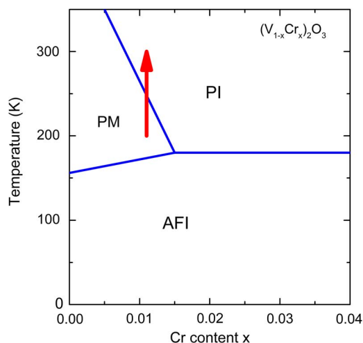
Figure 1. Phase diagram of (V_{1-x}Cr_x)_2O_3 including the AFI, the PM and the PI phases. Adapted with permission. [2] Copyright 2019, American Physical Society. The red arrow indicates that in the present experiments, the PM–PI phase composition was changed by increasing the temperature.
