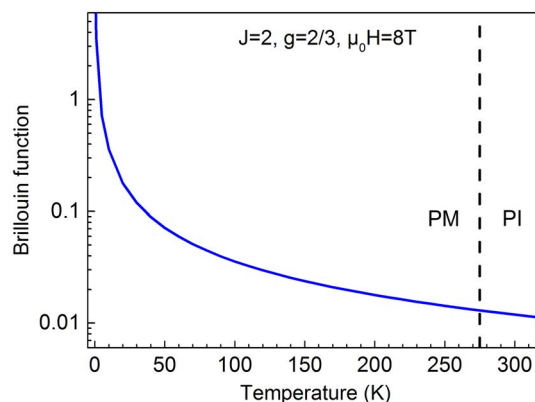
Figure 2. Brillouin function for V^{3+} (3d^2) with total angular momentum J = 2 , g -factor g = 2/3 , and magnetic flux density \mu_0 H = 8 \text{ T} . Since the PM–PI two-phase region exists at temperatures around 275 K (dashed line), the aligned paramagnetic moments are reduced by about two orders of magnitude compared with low temperatures of a few Kelvin.
