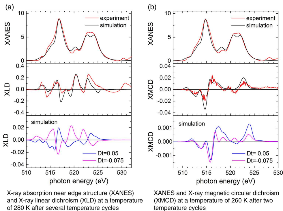
Figure 3. a) XLD, b) XMCD, and corresponding XANES spectra at the vanadium L_{2,3} edges in the PM–PI two-phase region of (V_{1-x}Cr_x)_2O_3 with x = 0.011 . The measurements (red lines) are compared with CTM4XAS simulations (black lines). The simulated XLD and XMCD spectra each consist of two spectra with Dt = 0.05 (blue lines) and Dt = -0.075 (magenta lines) weighted with a ratio of 4:6. For these XLD, XMCD, and corresponding XANES spectra, the same values of the crystal field parameters were used.
