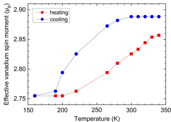
Figure 6. Estimated local spin moment plus the dipole moment of the spin density distribution 7\langle T_z \rangle of vanadium versus temperature while heating (red squares) and cooling (blue circles).
