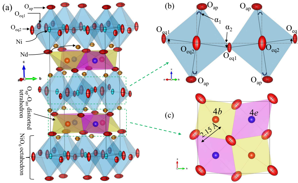
FIG. 1. (a) Perspective view of the tetragonal unit cell of \text{Nd}_2\text{NiO}_{4.11} in the P4_2/nm space group, showing two distinct tetrahedral sites 4b ( 3/4, 1/4, 1/4 ) (red spheres) and 4e ( 1/4, 1/4, z \sim 1/4 ) (blue spheres) accessible for extra oxygen atoms, while only the 4b Wyckoff site with point symmetry \bar{4} is occupied and the 4e tetrahedral site with point symmetry 2.mmm being entirely empty. Note that on average only 1/2 excess oxygen atom is present per unit cell, i.e., only 11% of 4b sites are filled in \text{Nd}_2\text{NiO}_{4.11} . (b) [110]/[001] projection of \text{NiO}_6 octahedral layer at z = 0.5 showing specifically the \text{NiO}_6 octahedron tilt pattern about the [110] axis. (c) [100]/[010] projection of the two \text{O}_{\text{int}}(\text{O}_{\text{ap}})_4 tetrahedrons with Wyckoff positions 4e and 4b showing inhaling and exhaling behavior of the empty (pink) and occupied (yellow) tetrahedra, respectively.
