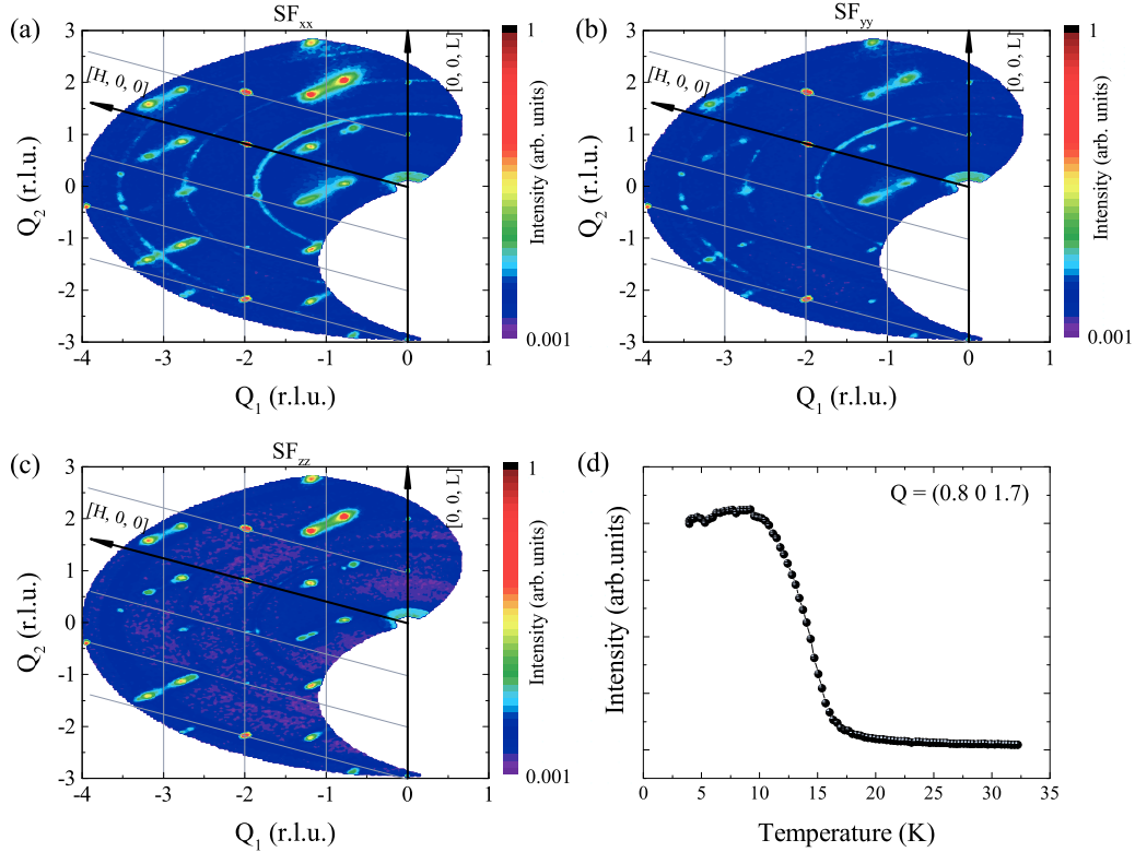
FIG. 8. Polarized neutron measurements of a Cu 2 CoSiO 5 single crystal. (a)–(c) The neutron scattering intensities within the spin-flip channels (a) SF_{xx} , (b) SF_{yy} , and (c) SF_{zz} detected within the reciprocal plane spanned by \mathbf{Q}_1 = (-1 \ 0 \ 0.4) and \mathbf{Q}_2 = (0 \ 0 \ 1) . Here, the x , y , and z directions are parallel to the average \mathbf{Q} , and perpendicular to the average \mathbf{Q} within the scattering plane and out of the scattering plane, respectively. The flipping ratio amounts to \sim 25 and intensities were not corrected for imperfect neutron polarization. Note, that the DNS spectrometer has a relaxed resolution in out-of-plane (here: K ) direction. (d) The temperature dependence of a (0.8 \ 0 \ 1.7) magnetic peak measured in the SF_{xx} channel.
