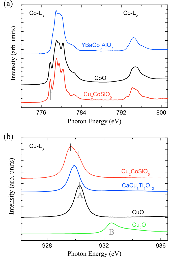
FIG. 5. (a) The \text{Co-L}_{2,3} XAS spectra of \text{Cu}_2\text{CoSiO}_5 and \text{CoO} with \text{Co}^{2+} ions in an octahedral coordination and \text{YBaCo}_3\text{AlO}_7 (from Ref. [12]) with \text{Co}^{2+} in a tetrahedral coordination. (b) The \text{Cu-L}_3 XAS spectra of \text{Cu}_2\text{CoSiO}_5 and of \text{Cu}_2\text{O} , \text{CuO} , and \text{CaCu}_3\text{Ti}_4\text{O}_{12} (from Ref. [16]) for comparison.
