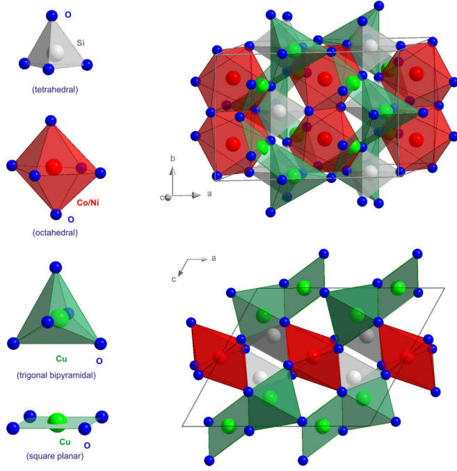
FIG. 4. Crystal structure of \text{Cu}_2\text{MSiO}_5 ( M = \text{Co}, \text{Ni} ). The oxygen coordination of the metal ions is shown on the left side, and the unit cell of \text{Cu}_2\text{MSiO}_5 for two different viewing directions (perpendicular and parallel to the chains running in the b direction) is shown on the upper and lower right.
