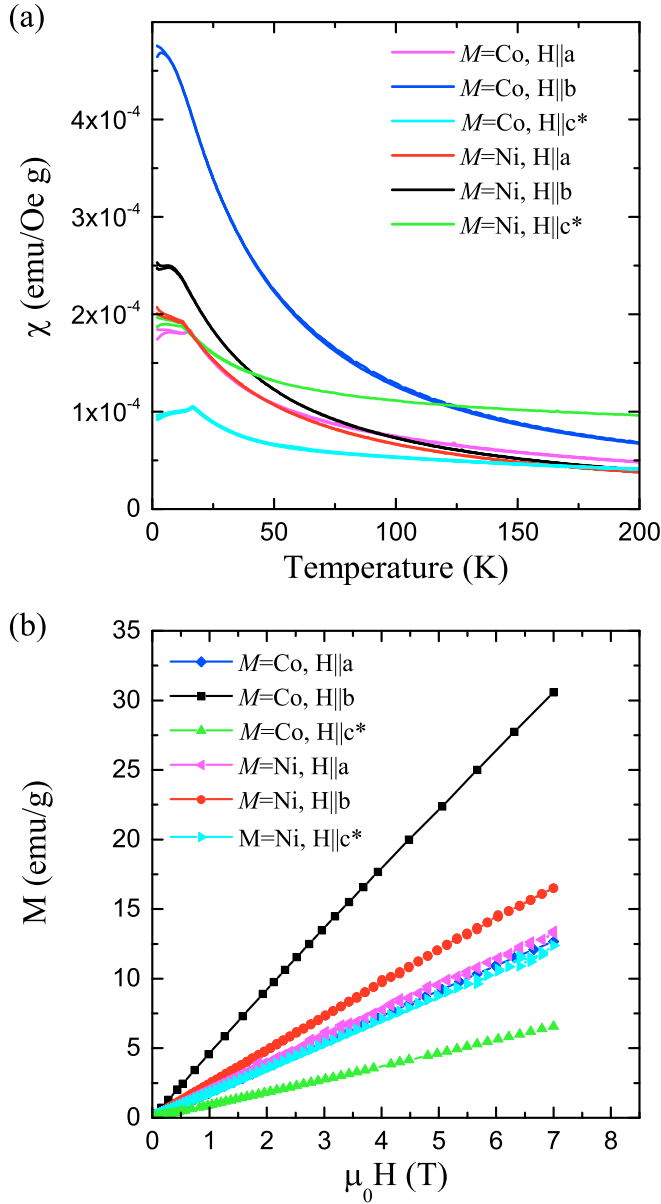
FIG. 6. (a) Temperature dependence of the magnetic susceptibility of \text{Cu}_2\text{MSiO}_5 ( M = \text{Co}, \text{Ni} ) for field-cooled and zero-field-cooled measurement conditions in magnetic fields of \mu_0 H = 0.1 and 0.25 T for M = \text{Co} and \text{Ni} respectively. The field was applied along the crystallographic a and b directions as well as the c^* direction, which is perpendicular to a and b within this monoclinic system ( a \perp b \perp c^* ). (b) Magnetization measurements of \text{Cu}_2\text{MSiO}_5 at 2 K.
