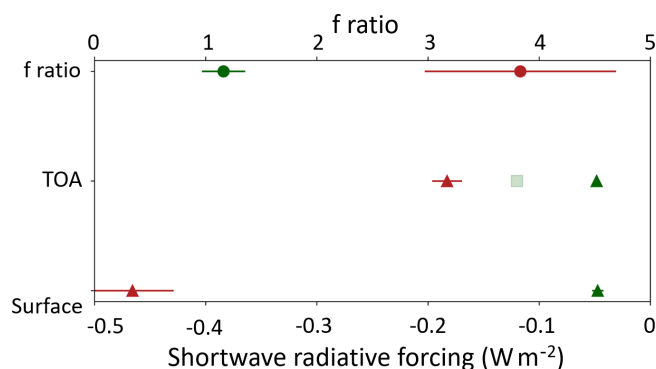
Figure 6. Daily average clear-sky top of the atmosphere (TOA) and surface direct radiative forcing (triangles), and f ratio (dots), for the mean fire plume and ATAL profiles of Fig. 2a. Green represents the calculations for the ATAL, red for the fire. The variability of the SSA in our calculations is reflected by the error bars. The clear-sky TOA radiative forcing estimation for the July–August ATAL of Vernier et al. (2015) is also shown (semi-transparent green square).
