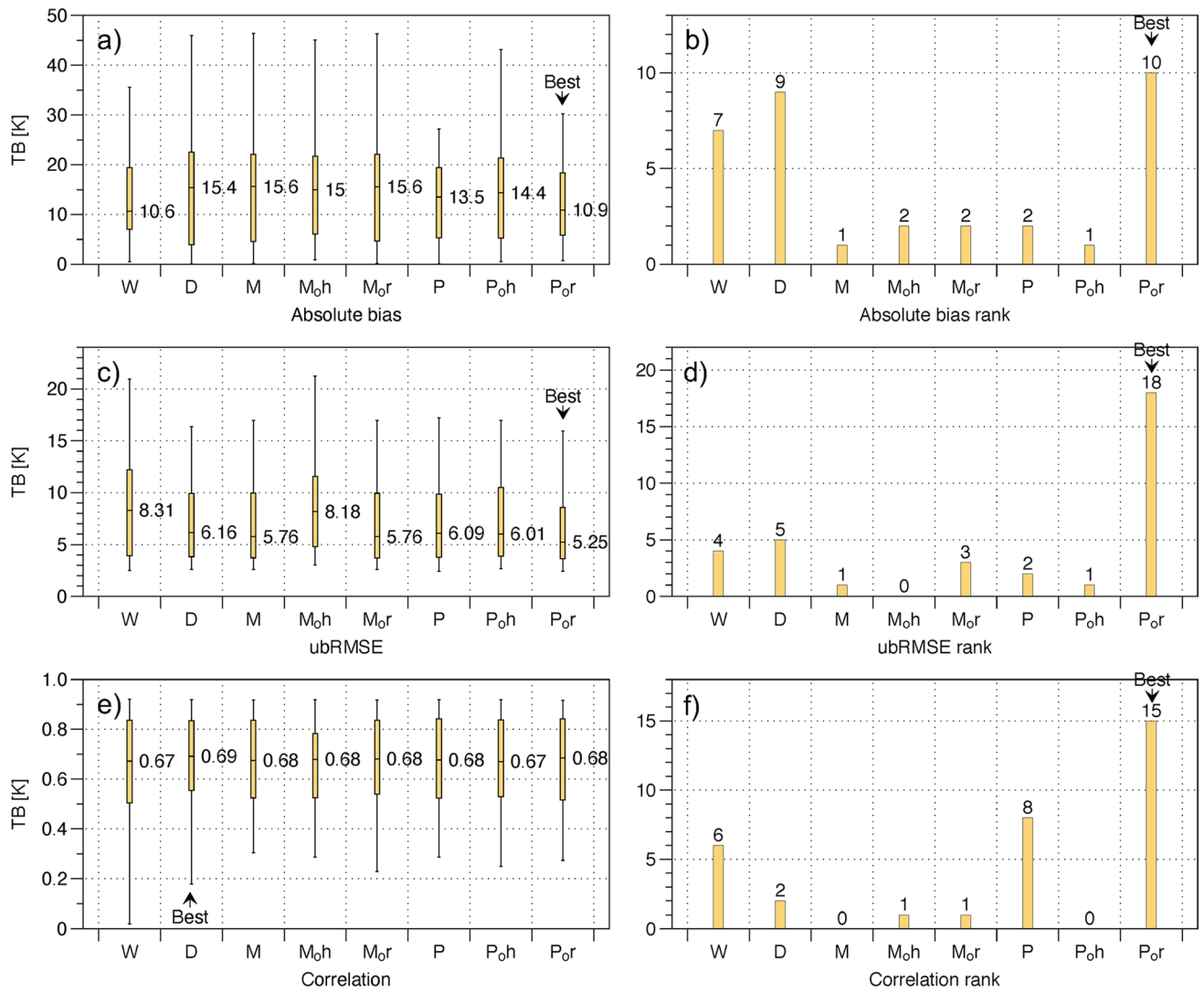
Fig. 10. Spatially averaged brightness temperature (Tb) evaluation scores for the 35 International Soil Moisture Network sites in Table 3, calculated for the period from 1 June to 30 Sept. 2015 (left), and the number of counts for first rank among the tested models (right). The models included Wang and Schmugge (1980) (W), Dobson et al. (1985) (D), Mironov et al. (2009) (M) and with organic matter (OM) input from the Harmonized World Soil Database (FAO, 2012) (M 0h ) and the SoilGrid1km database (Hengl et al., 2014) (M 0r ), and (Park et al., 2017) with wilting point and porosity classified by USDA soil classification (P) and with wilting point (Eq. [1]) functions and OM input from the SoilGrid1km database (P 0r ) or with wilting point (Jin et al., 2017) and porosity (Wösten et al., 1999) functions and OM input from the Harmonized World Soil Database (P 0h ).
