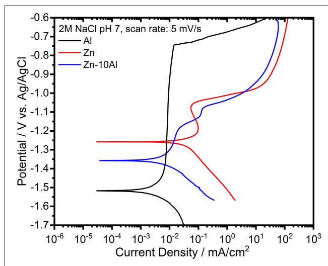
FIGURE 7 | Potentiodynamic polarization curves of pure Al and Zn, and Zn-10Al alloy electrodes in 2M NaCl solutions with pH 7. The scans for each electrode was initiated at cathodic potentials toward the anodic direction with a scan rate of 5 mV/s.
