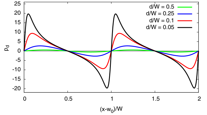
FIG. 5. The grain boundary shape equation (16) in its dimensionless form, p_d(x/W) = p(x/W)W\beta/[\varepsilon_0 R^2(1 + \nu)] . Different values of d/W are used to show the effect of these two parameters on the grain boundary deformation.
