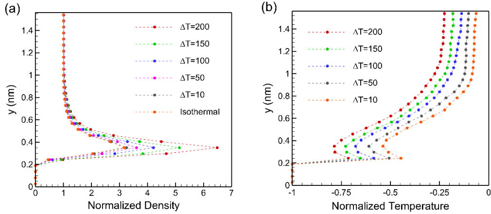
Fig. 8. Variation of normalized density (a) and normalized temperature (b) in 1.5 nm from the lower wall for various temperature differences between the walls.
