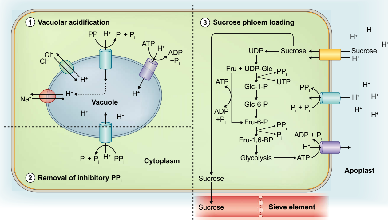
Fig. 3 A variety of roles for the vacuolar proton-pumping pyrophosphatase. A generic plant cell showing the variety of ways the vacuolar proton pumping pyrophosphatase (H + -PPase) can provide an alternative source of energy during salinity stress. (1) Vacuolar acidification. Localized to the tonoplast, the vacuolar H + -PPase (blue) will use energy released from the hydrolysis of PP i to orthophosphate (P i ) to pump protons (H + ) into the vacuole. Along with vacuolar ATPases (purple), vacuolar H + -PPases establish an electrochemical potential for H + across the tonoplast, which is used by other vacuolar transporters (red & brown) to sequester Na + and Cl - into the vacuole. (2) Removal of inhibitory pyrophosphate (PP i ). Vacuolar H + -PPases regulate PP i concentrations in the cytosol. Accumulation of PP i in the cytosol, particularly in younger tissues, can inhibit PP i -dependent metabolic pathways, such as gluconeogenesis and the Smirnov–Wheeler pathway. (3) Enhancing sucrose transport from source to sink tissues. In phloem companion cells, H + -PPases are shown to be localized to the plasma membrane, where it is hypothesized they synthesize PP i from orthophosphate. This additional PP i is used to enhance sucrose metabolism in these cells, thereby generating more ATP to pump protons into the apoplast which can be used by sucrose transporters, ultimately enhancing sucrose transport into sieve elements. Not all of these processes will be occurring in all cells at all times, and some may be cell-type specific. Figure modified from Khadilkar et al. (2016) and Schilling et al. (2017).
