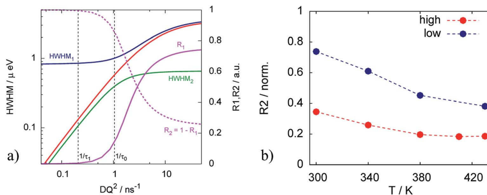
Fig. 6 (a) Widths of the two components I_1 and I_2 of the trap model and their spectral weights at T = 340 K. Red line is the width \Gamma of the free PA. (b) Amount of the trapped protons (estimated from the R_2 at the highest Q ) in the catalytic layer for different doping levels.
