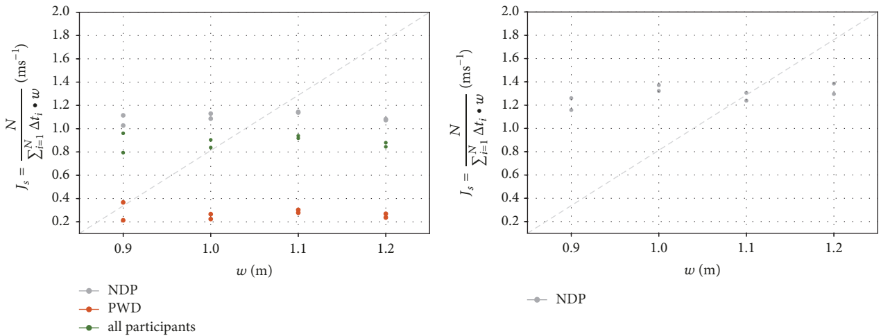
FIGURE 9: Comparison of specific flows for bottleneck studies considering different subpopulations in a bottleneck. Reference data is obtained from [37].
