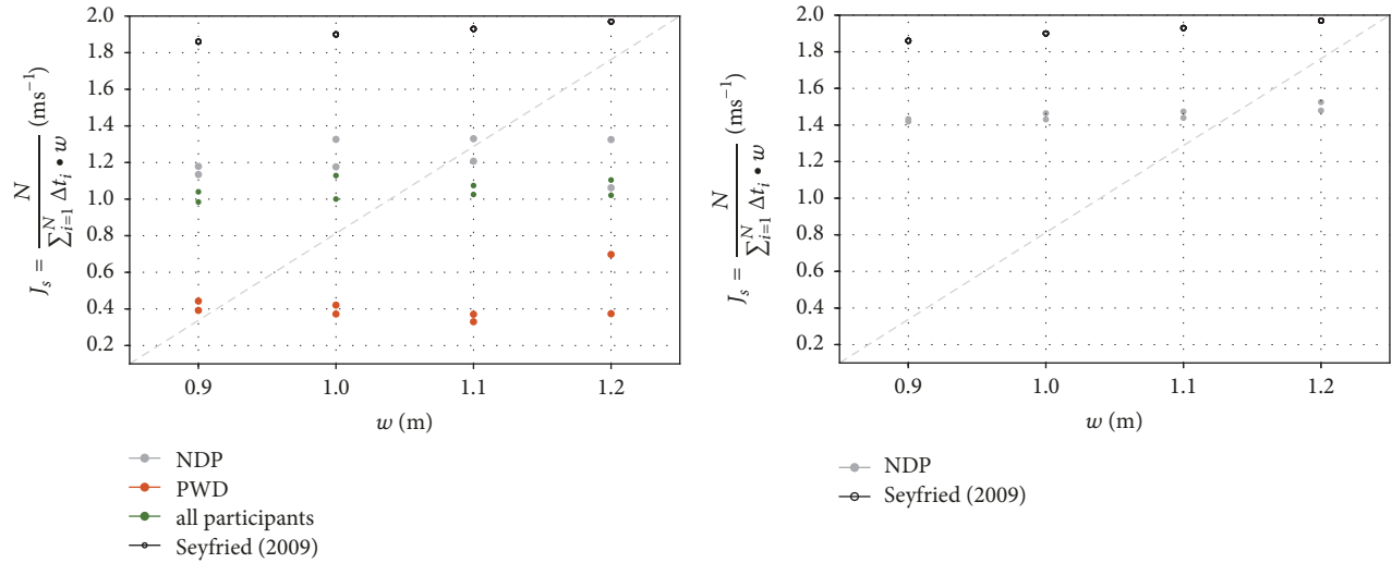
FIGURE 9: Comparison of specific flows for bottleneck studies considering different subpopulations in a bottleneck. Reference data is obtained from [37].
