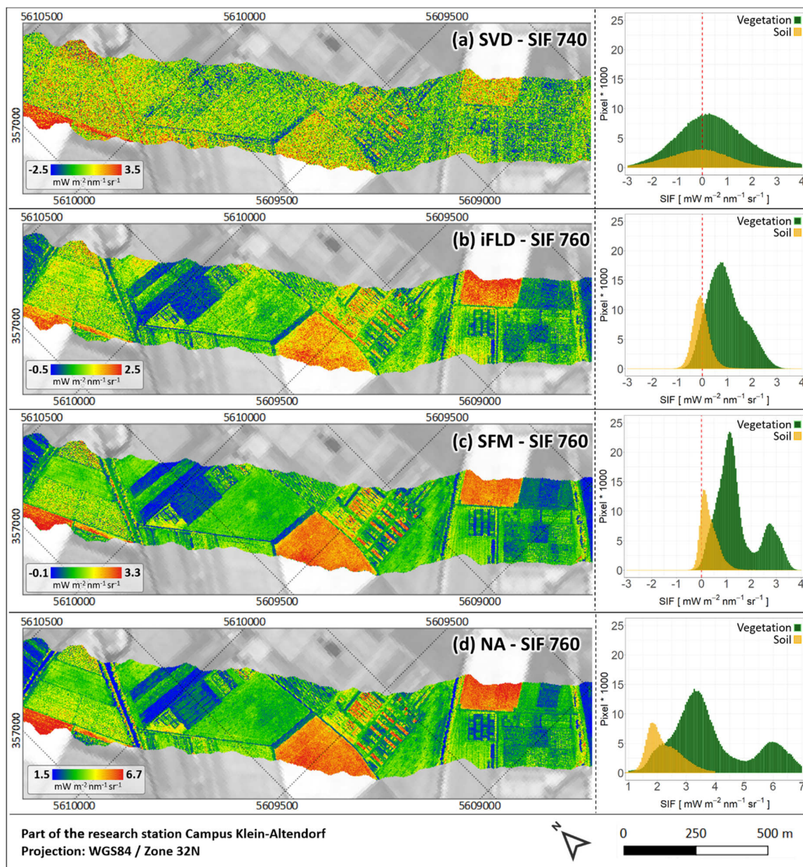
Figure 9. SIF maps derived for the O_2 -A absorption feature, showing a part of the agricultural research station Campus Klein-Altendorf, acquired on 29 June 2018 and corresponding pixel value distributions for vegetation and soil pixels: (a) results of the SVD method; (b) results of the iFLD method; (c) results of the SFM method; (d) results of the NA method.
