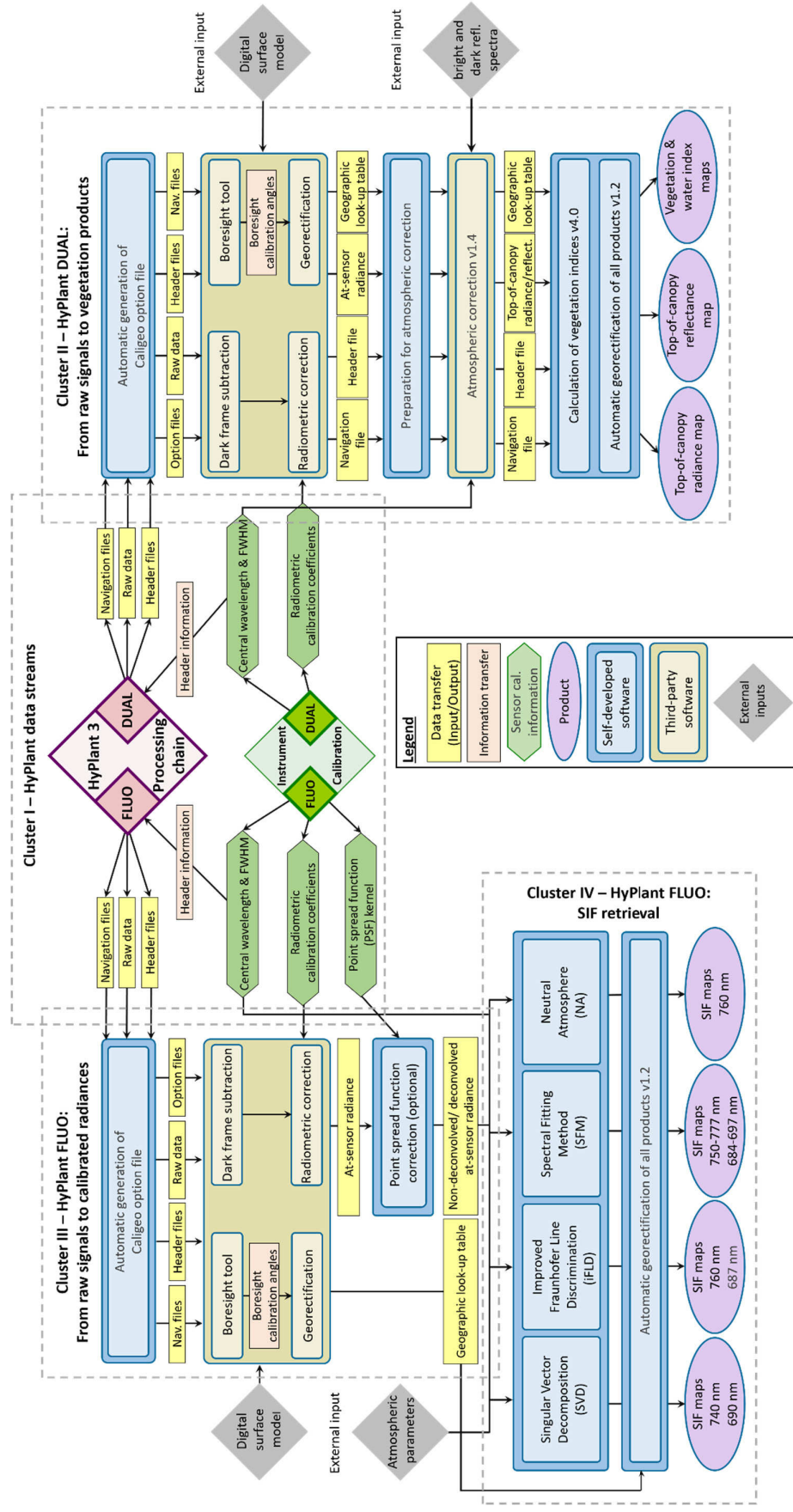
Figure A1. Overview of the HyPlant processing chain consisting of the four processing cluster.
