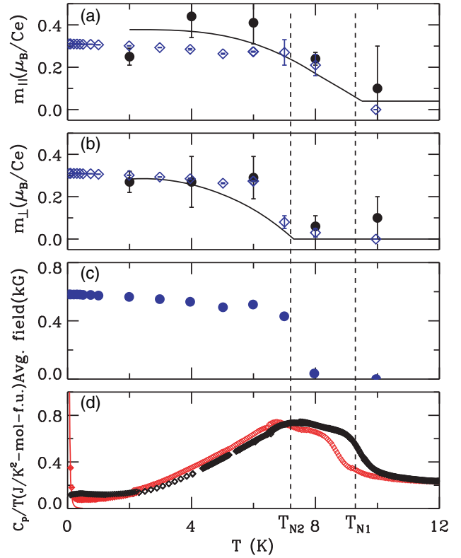
FIG. 2. Temperature dependence of (a) the longitudinal ( m_a ) and (b) the transverse moments ( m_c for high T and m_b for low T phase). Black dots were extracted from Rietveld fits to neutron diffraction data. The 2 and 8 K data points were averaged over two chopper settings. Blue diamonds were inferred from \mu SR fits. The solid lines are guides to the eye. (c) Temperature dependence of the averaged static field. (d) Specific heat C_p/T in zero field and for \mu_0 H = 14 T. The upturn in C_p/T at 14 T is due to the nuclear spin contributions as indicated by the solid red line.
