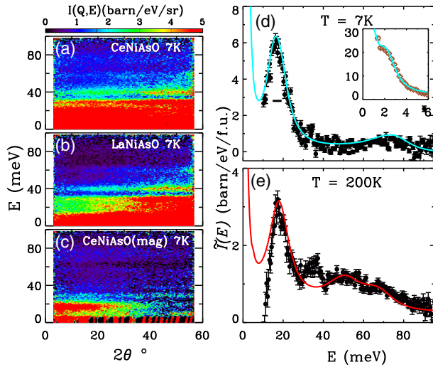
FIG. 4. Normalized inelastic spectrum with incident energy E_i = 100 \text{ meV} (black dots) for (a) CeNiAsO and (b) the non-magnetic reference LaNiAsO. (c) The T = 7 \text{ K} difference spectrum: \tilde{I}(Q, E) = I_{\text{Ce}} - r I_{\text{La}} where r = \sigma_{\text{CeNiAsO}}/\sigma_{\text{LaNiAsO}} . (d), (e) Momentum-integrated scattering at T = 7 \text{ K} and 200 \text{ K} inferred from the method in Refs. [38–40]. The horizontal black bar indicates energy resolution. The inset in (d) shows a magnetic excitation at 2 \text{ meV} in the ordered state with E_i = 50 \text{ meV} (brown dots). The cyan and red solid lines were calculated for the crystal field model described in the text.
