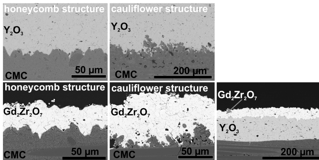
Figure 8. SEM images of APS Y_2O_3 and Gd_2Zr_2O_7 coatings on laser structured Ox/Ox CMC substrates after thermal cycling ( 4 \times 20 h at 1200^\circ C ).
