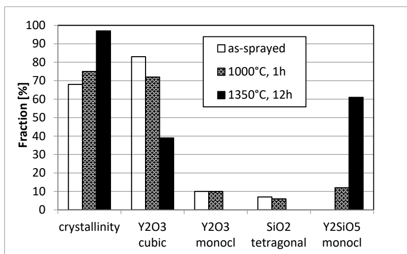
Figure 11. Phase evolution in APS \text{Y}_2\text{SiO}_5 coatings (condition D) after heat-treatment.
