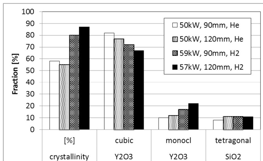
Figure 9. Phase evaluation of 4 \text{Y}_2\text{SiO}_5 coatings (caption indicate power, stand-off distance and secondary gas).
