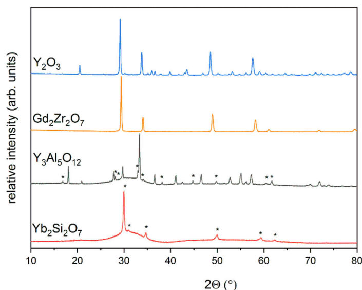
Figure 3. XRD measurements of \text{Y}_2\text{O}_3 , \text{Gd}_2\text{Zr}_2\text{O}_7 , \text{Y}_3\text{Al}_5\text{O}_{12} and \text{Yb}_2\text{Si}_2\text{O}_7 coatings in the as-sprayed state, peaks of secondary phases are marked with *.
