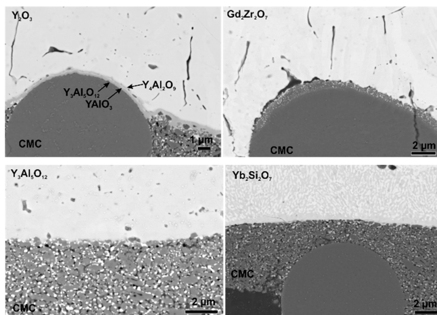
Figure 5. SEM images of the coating substrate interface of \text{Y}_2\text{O}_3 , \text{Gd}_2\text{Zr}_2\text{O}_7 , \text{Y}_3\text{Al}_5\text{O}_{12} and \text{Yb}_2\text{Si}_2\text{O}_7 coatings on Ox/Ox CMCs after thermal treatment.
