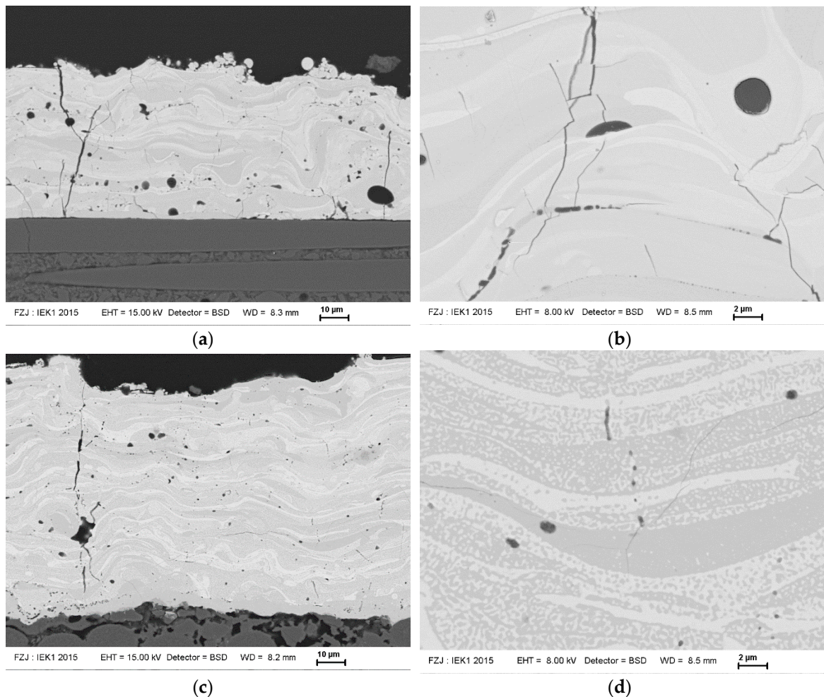
Figure 10. SEM micrographs of plasma-sprayed \text{Y}_2\text{SiO}_5 coatings (condition D) in the as-sprayed (a,b) and annealed (c,d, 1350°C, 12h) condition.
