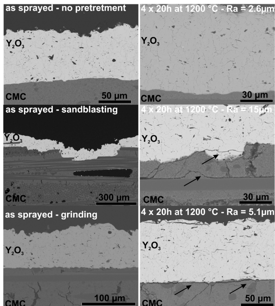
Figure 6. SEM images of APS- \text{Y}_2\text{O}_3 coatings on Ox/Ox CMCs with and without mechanical pre-treatment before and after thermal cycling.
