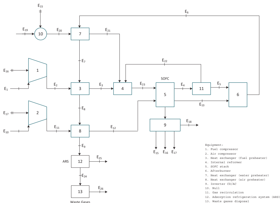
Figure 1. Schematic diagram of the solid oxide fuel cell-vapor absorption refrigeration hybrid system.
