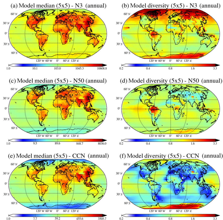
Figure 10. Global distributions of the annual multi-model median concentrations of N 3 , N 50 and CCN 0.2 (cm -3 ) for the year 2011 (a, c, e, respectively) and the corresponding diversities (b, d, f, respectively; calculated as the ratio of standard deviation to the mean of the models).
