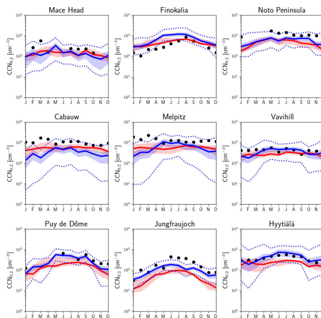
Figure 5. Monthly average \text{CCN}_{0.2} based on HadGEM3-UKCA perturbed parameter ensemble simulations for the year 2008. The solid blue line shows the mean of the sample of 260 000 model variants from the emulator for each month and station. The shaded blue area shows the range of this mean plus and minus 1 standard deviation, while the blue dashed lines show the minimum and maximum sampled values. The red line shows the MMM results (mean of the years 2011–2015 shown in Fig. 2), and the shaded red area corresponds to the 25 % and 75 % quartiles. The \text{CCN}_{0.2} values obtained from observational data are shown by symbols (mean of the available data).
