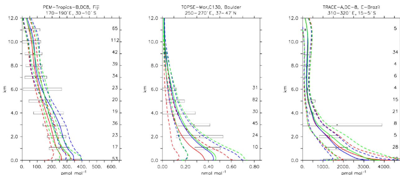
Figure 13. Comparison of simulated CH 2 O vertical profiles by using the CBA (red), MOC (blue) and MOZ (green) chemistry versions against aircraft data (black). Line styles and symbols have the same meaning as in Fig. 12.
