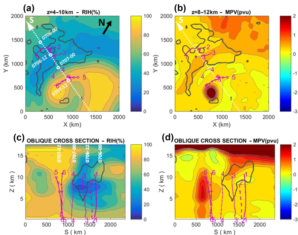
Figure 7. Composites of ERA-5 reanalyses data from 6 July at 00:00 UTC to 7 July at 12:00 UTC in the domain shown in Fig. 5a. Above are horizontal distributions of (a) relative integrated humidity (RIH) between 4 and 10 km altitude (in %) and (b) mean potential vorticity (MPV) between 8 and 12 km altitude (in PVU; = 10^{-6} \text{ m}^2 \text{ s}^{-1} \text{ K kg}^{-1} ). North is indicated in (a). The dotted white line ( S axis) represents the pseudo-trajectory of TPE airport in the frame moving with Typhoon Nepartak (successive times are indicated). Below are vertical cross sections of (c) RIH (in %), and (d) MPV (in PVU), averaged across \pm 500 km along this oblique S line. The solid black contours encompass mean downward velocities < -1 \text{ cm s}^{-1} between 6 and 10 km altitude. The purple lines 1 to 6 indicate the tracks of IAGOS aircraft during selected take-offs and landings on 6–7 July.
