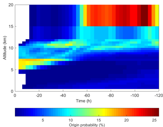
Figure 8. Time–altitude distribution of probability (in %) of back-trajectory origin when initiated within the domain 24–26° N, 120–122° E (4–10 km altitude), on 6 July at 12:00 UTC.
