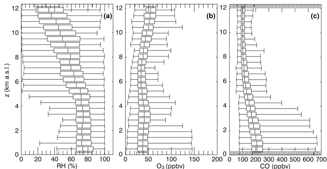
Figure 1. Boxplots showing first percentile, first quartile, median, third quartile and 99th percentile of (a) relative humidity (RH; limited to 100 %), (b) ozone ( \text{O}_3 ) and (c) carbon monoxide (CO) between 0 and 12 km altitude from IAGOS measurements during take-off from and landing to TPE over the time periods 1 July to 31 October in 2012–2016.
