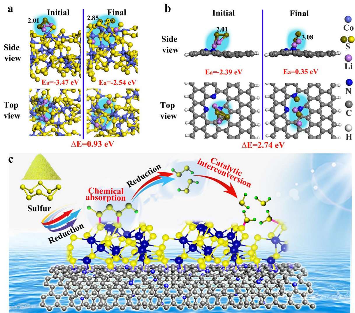
Figure 5. The absorption energy ( E_a ) and dissociation energy ( \Delta E ) of \text{Li}_2\text{S}_2 on the surface of (a) \text{CoS}_3 and (b) NCNT. (c) Schematic illustration of the reaction process of sulfur on the \text{CoS}_3 catalyst.
