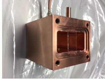
Fig. 2 First measurement prototype. A 15 \times 8 \times 0.33 \text{ mm}^3 sapphire crystal is anchored using cryogenic grease to the copper holder, acting also as waveguide. Three GrAl resonators (not visible because of the very small size) are deposited in the center of the sapphire crystal. Color figure online.
