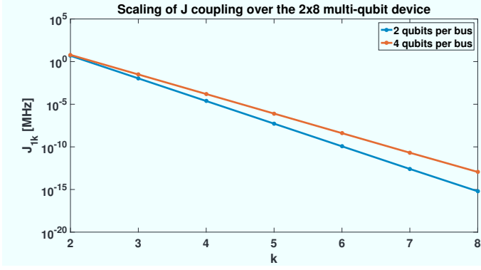
Figure 5: Exponential decay of the J_{1k} coupling rate for k = 2, \dots, 8 as measured from the first qubit Q_1 to the right in the upper rows in Figs. (3) and (4) as a function of qubit index k . J_{12} is -4.9 \text{ MHz} and -6.1 \text{ MHz} in the devices in Figs. (3) and (4), respectively.
