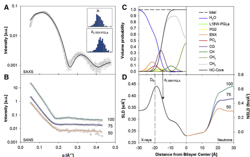
FIGURE 2 SDP analysis of POPE/POPG (3:1 mol/mol) in the presence of L18W-PGLa (P:L = 1:200). (A) and (B) show the calculated model fits from averaged parameters (solid lines) for SAXS and SANS data, obtained from 400 independent optimization runs. Insets in (A) show histograms of the area per unit cell, A_U , and the position of the peptide in the bilayer, z_p . (C) shows the volume probability distribution of the bilayer, and panel (D) displays the corresponding electron and neutron scattering length densities. The arrow indicates location of z_p , and the dashed line shows the position of D_B/2 . To see this figure in color, go online.
