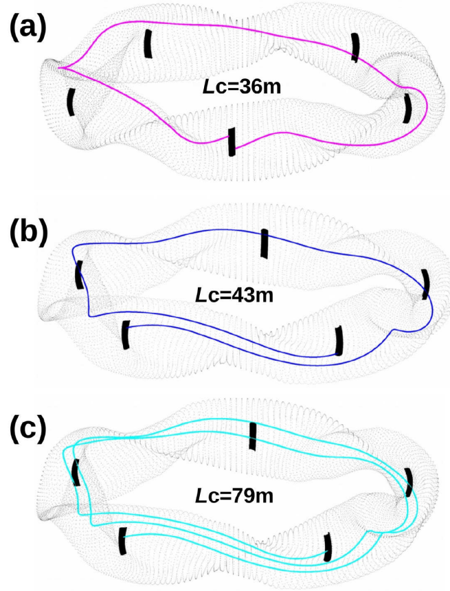
Figure 3: Magnetic field lines representing the three different types of magnetic flux bundles in the SOL. (a) A field line starts on a limiter and hits the same limiter after one toroidal turn (1 turn, L_C \approx 36\text{m} ). (b) A field line starts on a limiter and hits after one toroidal turn the next neighbouring limiter (1.2 turns, L_C \approx 43\text{m} ). (c) A field line starting on one limiter performs two toroidal turns until hitting the next neighbouring limiter (2.2 turns, L_C \approx 79\text{m} ).
