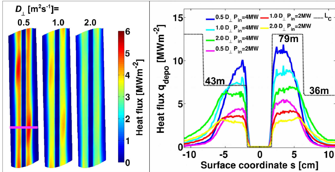
Figure 8: Left: 2-D limiter heat flux deposition for a transport parameter scan for a pure hydrogen plasma at n_{\text{LCFS}} = 9 \cdot 10^{18} \text{m}^{-3} , P_{\text{in}} = 2 \text{MW} , D_{\perp} = 0.5, 1.0, 2.0 \text{m}^2 \text{s}^{-1} , \chi_{\perp, e, i} = 3D_{\perp} . Right: 1-D surface scan of the deposited heat flux at Z = -0.2 \text{m} for a transport and power parameter scan at n_{\text{LCFS}} = 9 \cdot 10^{18} \text{m}^{-3} , P_{\text{in}} = 2 \text{MW}, 4 \text{MW} , D_{\perp} = 0.5, 1.0, 2.0 \text{m}^2 \text{s}^{-1} , \chi_{\perp, e, i} = 3D_{\perp} extracted at Z = -0.2 \text{m} , magenta mark, left.
