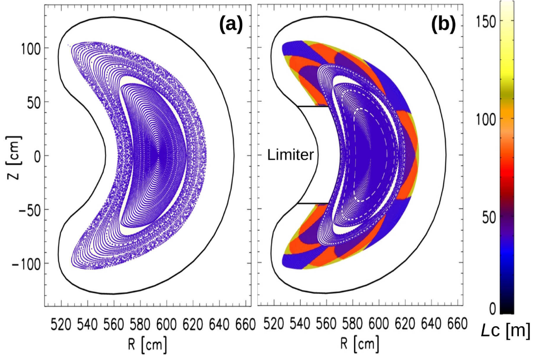
Figure 1: (a) Poincare plot of the vacuum magnetic field at the bean shaped symmetry plane ( \phi_{tor} = 0^\circ ) within the vessel (black solid line). (b) Target-to-target connection lengths ( L_C ) topology arising once the five graphite inboard limiters inserted open the field lines of the boundary magnetic field. The SOL domain relevant for plasma transport consists of three L_C : 36m (blue), 43m (purple) and 79m (orange).
