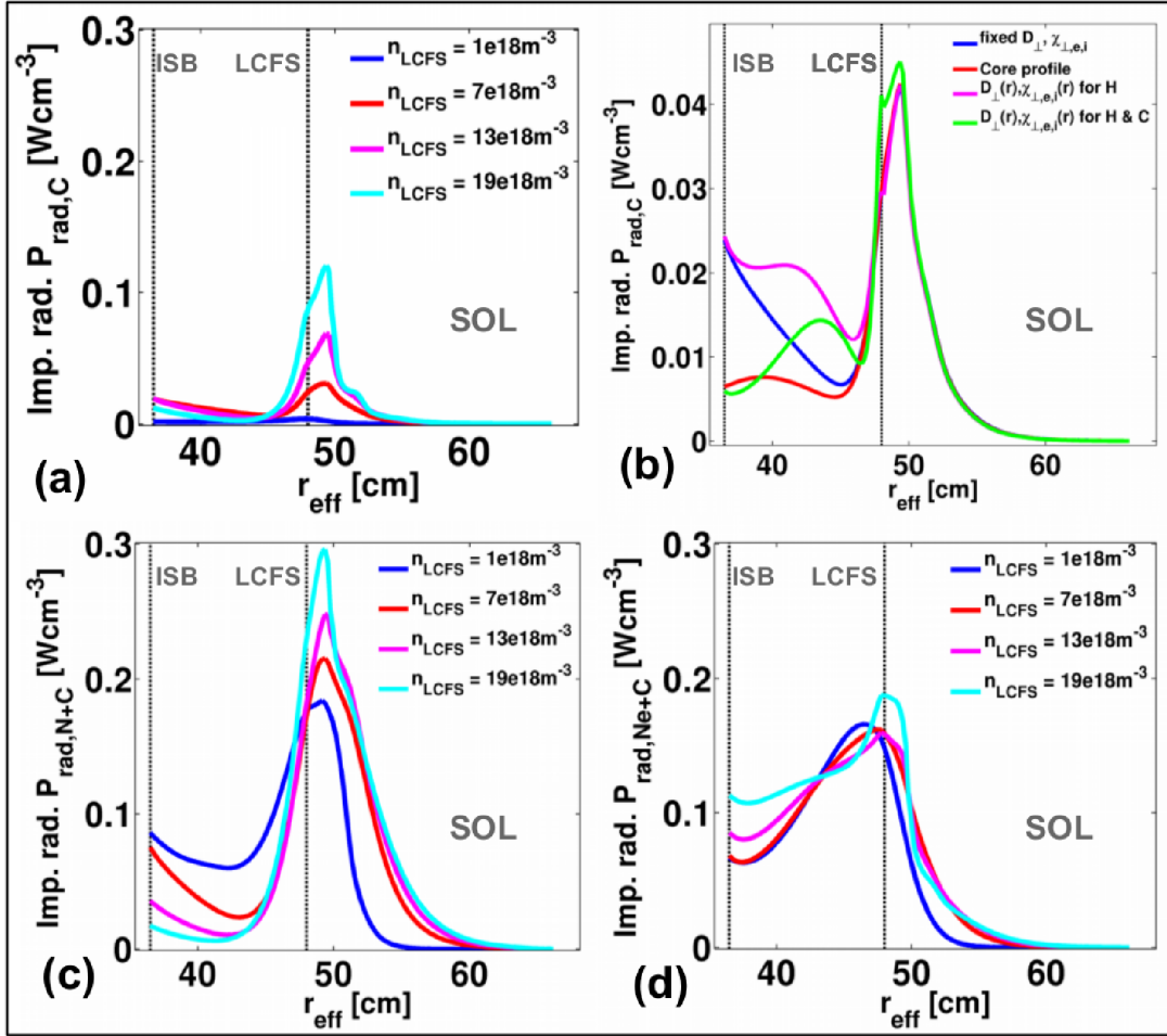
Figure 11: Radial distribution of total impurity radiation for the density scan at P_{\text{in}} = 4\text{MW} . (a) Intrinsic carbon eroded from the limiter, (b) intrinsic carbon for different transport conditions at fixed n_{\text{LCFS}} = 9 \cdot 10^{19} \text{ m}^{-3} , (c) seeded nitrogen (including intrinsic carbon), (d) seeded neon (including intrinsic carbon). The black dotted lines indicate ISB and LCFS (relevant for the boundary conditions).
