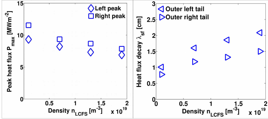
Figure 7: Left: Maximum deposited peak heat fluxes P_{\text{peak}} and right: limiter surface deposition decay lengths \lambda_{\text{sf}} for four different density cases n_{\text{LCFS}} = 1 \cdot 10^{18} , 7 \cdot 10^{18} , 1.3 \cdot 10^{19} and 1.9 \cdot 10^{19} \text{m}^{-3} at P_{\text{in}} = 4 \text{MW} inferred from the 1-D profiles in figure 6.
