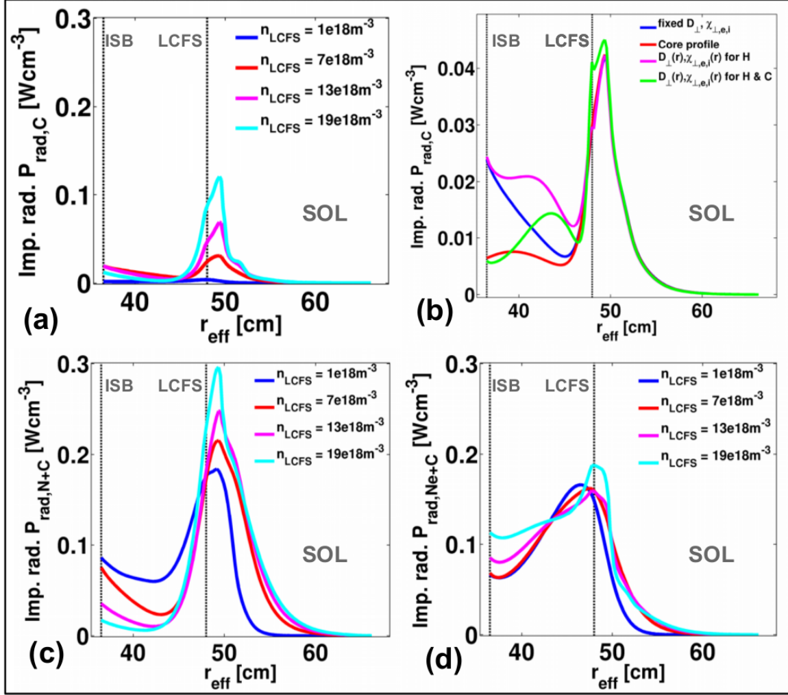
Figure 11: Radial distribution of total impurity radiation for the density scan at P_{in}=4\text{MW} . (a) Intrinsic carbon eroded from the limiter, (b) intrinsic carbon for different transport conditions at fixed n_{LCFS} = 9 \cdot 10^{19} \text{m}^{-3} , (c) seeded nitrogen (including intrinsic carbon), (d) seeded neon (including intrinsic carbon). The black dotted lines indicate ISB and LCFS (relevant for the boundary conditions).
