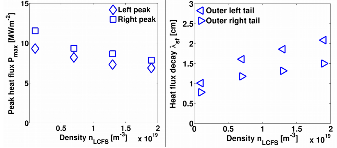
Figure 7: Left: Maximum deposited peak heat fluxes P_{\text{peak}} and right: limiter surface deposition decay lengths \lambda_{sf} for four different density cases n_{\text{LCFS}} = 1 \cdot 10^{18} , 7 \cdot 10^{18} , 1.3 \cdot 10^{19} and 1.9 \cdot 10^{19} \text{m}^{-3} at P_{\text{in}} = 4 \text{MW} inferred from the 1-D profiles in figure 6.
