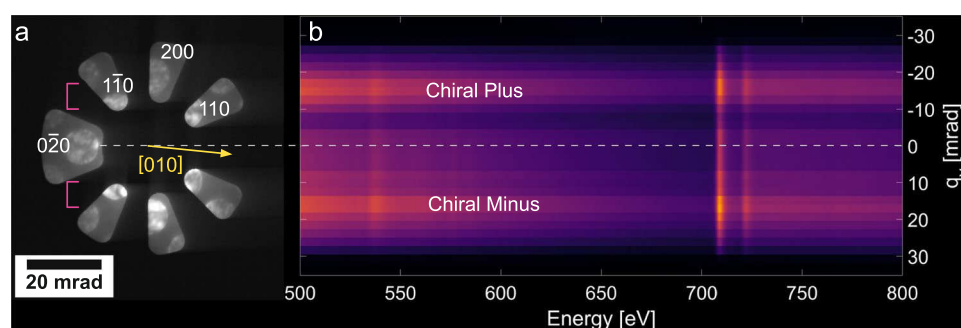
Figure 2. (a) Experimental diffraction pattern recorded on the GIF CCD showing the electron optical conditions. The probe was centered on the grain of interest (see Fig. 3). (b) 2D EELS spectrum acquired using the electron optical conditions presented in (a). The q_y axis represents the momentum transfer that would be expected for a slit oriented normal to the spectrometer dispersion plane. The oxygen edge visible at 532 eV comes from the \text{Al}_2\text{O}_3 capping layer and is primarily dominant in the background regions. The magenta brackets denote the angular span of the EMCD sign inversion on \text{Fe } L_3 observed in Fig. 9.
