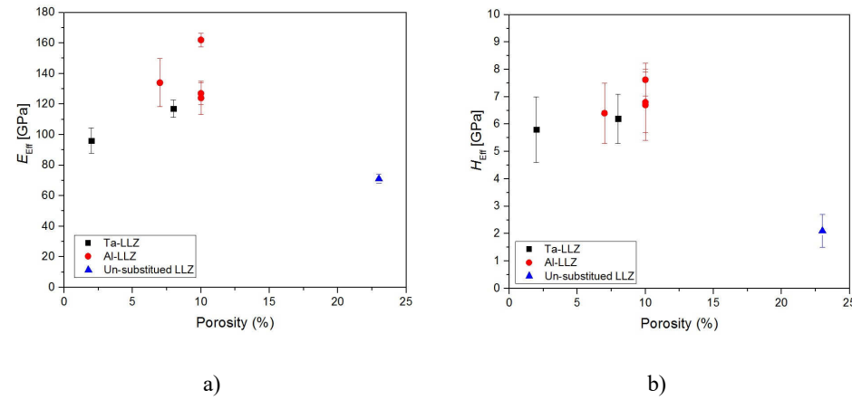
Figure 4.6- Effective mechanical properties (determined using high loads) plotted as function of porosity (a) effective elastic modulus ( E_{\text{eff}} ) (b) effective hardness ( H_{\text{eff}} ).
