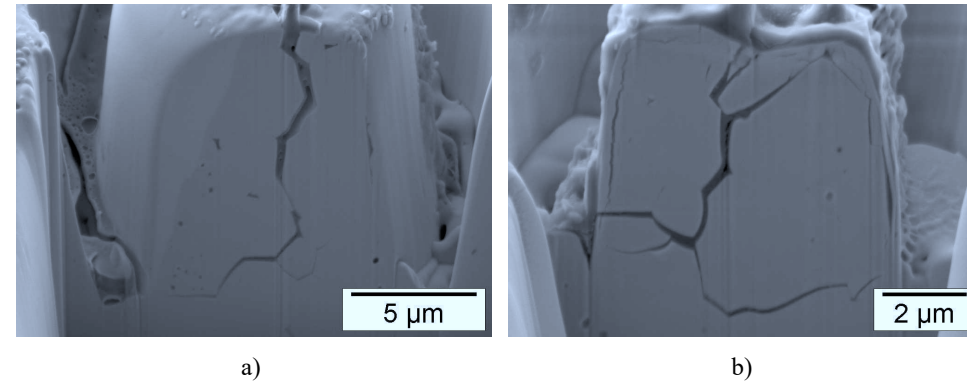
Figure 4.44 –SEM micrographs of cross-sectional FIB cut on HP-Al:LLZO-SG of a) pillar 5 (~10 \mu\text{m} diameter) b) pillar 9 (~5 \mu\text{m} diameter).
