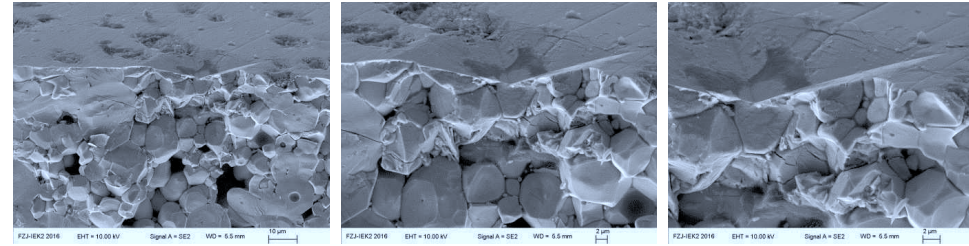
Figure 4.20- SEM micrographs of indented cross-section of 40Ta:LLZO-16h.
