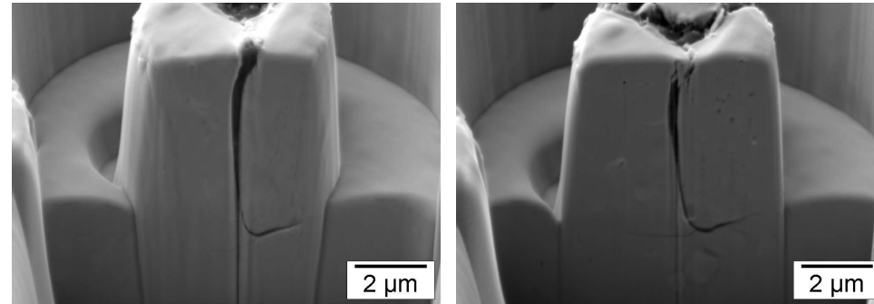
Figure 4.41- SEM micrographs of cross-sectional FIB cut of pillar H (~ 5 \mu\text{m} diameter) after indentation splitting.
