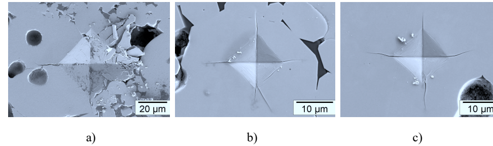
Figure 4.10- SEM micrographs of typical indentation marks at 1 N in a) 20Al:LLZO-20h; b) 20Al:LLZO-2h; c) 20Al:LLZO-40h.
