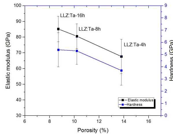
Figure 4.18-Influence of porosity on mechanical properties of 40Ta:LLZ.
