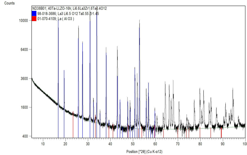
Figure 4.13- XRD spectra of LLZ:Ta-16h after sintering.
