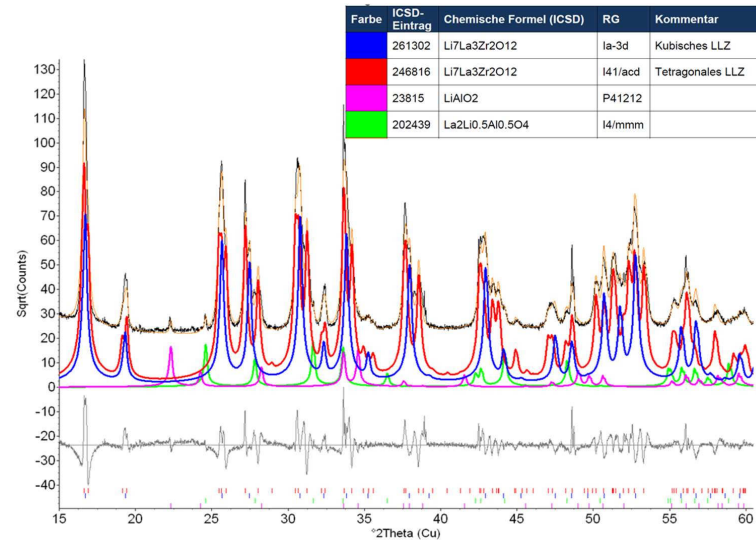
Figure 4.7- XRD pattern of 20Al:LLZ-2h.
