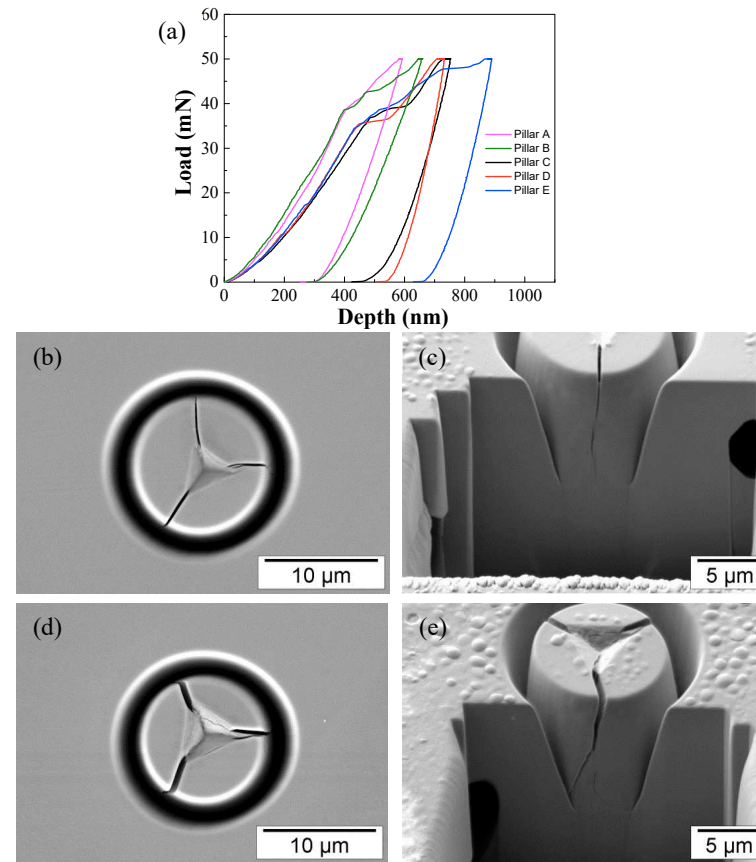
Figure 4.31- (a) Load-displacement curves of micro-pillar indentation splitting tests and some corresponding SEM-FIB images for (b), (c) front and side view of pillar A and (d), (e) front and side view of pillar B. It is worth notice that a blister-like surface morphology was only observed after further FIB milling for topological observation in (c, e). A featureless surface morphology was observed in (b, d) during and immediately after indentation.
