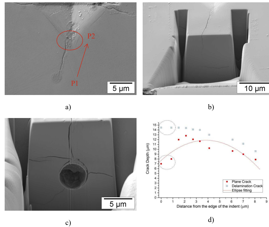
Figure 4.30- SEM micrographs of sample morphology after applying VIF test (a) selected crack for investigation: P 1 is the end of the imprinted, P 2 indicates 0 μm from the imprinted tip and red arrow indicate the direction of the FIB cutting (b-c) the extended cracks obtained from several SEM-FIB cross sectional, where the position P 1 and P 2 were located at the beginning and the end of the extended cracks. The crack depth vs. distance from the FIB cuts are plotted in (d), and the dash circle indicates the location of one large pore (radius ~ 2 μm).
