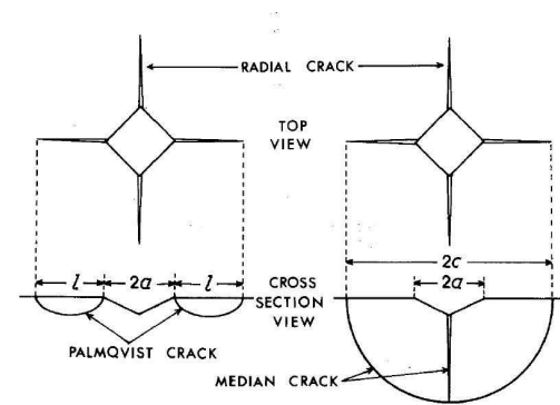
Figure 2.5- Schematic of Palmqvist cracks and median-radial cracks [114].
