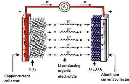
Figure 2.1- Schematic illustration of traditional lithium-ion battery [9].
