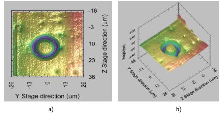
Figure 3.5- Scanned surface of HP-Al:LLZO-SG before testing a) plan view; b) 3D view of micro-pillar.
