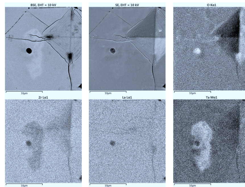
Figure 4.22- EDX mappings of the previous indentation affected by two indentations presented in previous figure.
