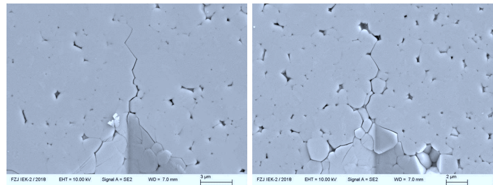
Figure 4.38- Crack deflection along the grain boundary sample HP-Al:LLZO-SG indentation load 1 N.
