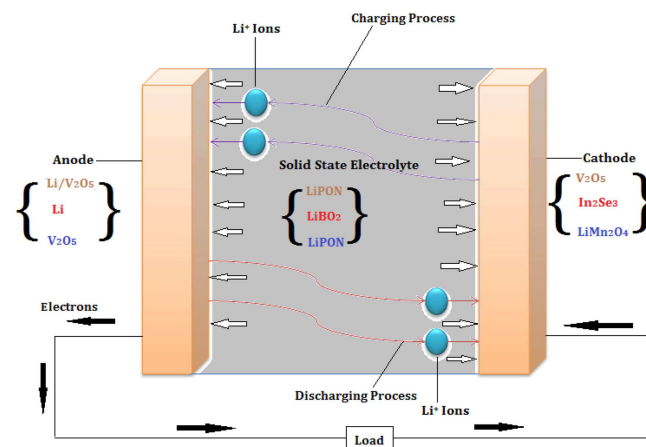
Figure 2.2- Schematic representation of a lithium based solid-state battery [8].
