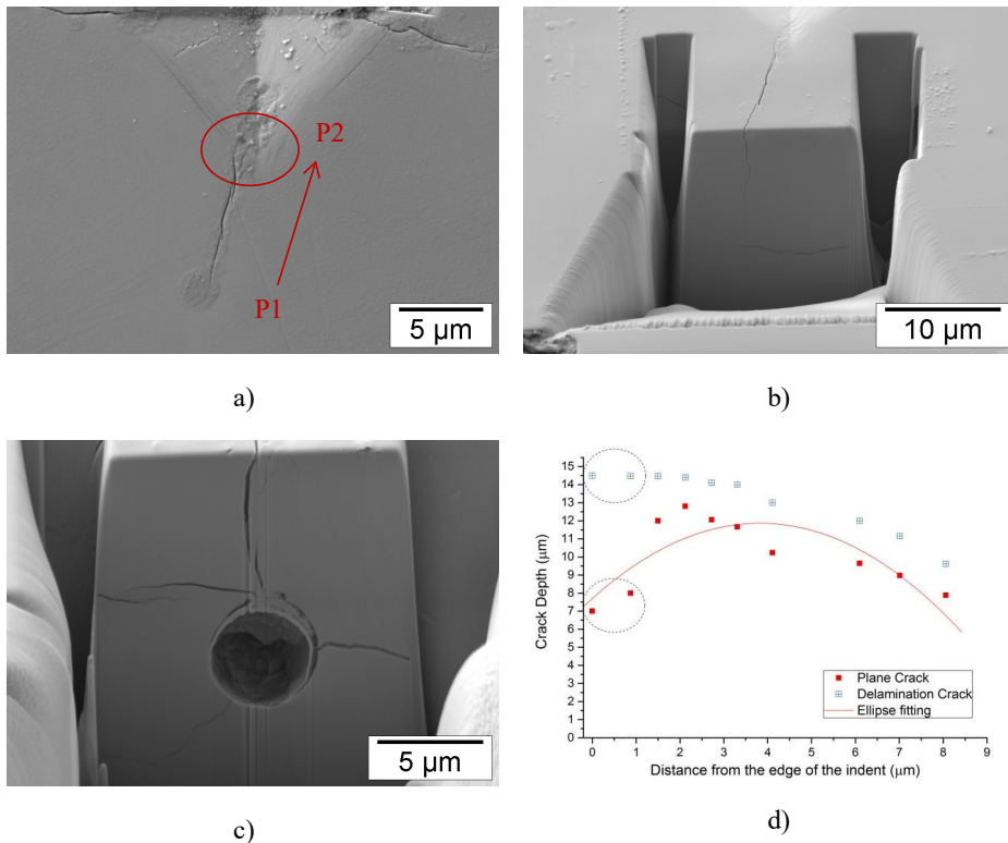
Figure 4.30- SEM micrographs of sample morphology after applying VIF test (a) selected crack for investigation: P 1 is the end of the imprinted, P 2 indicates 0 \mu\text{m} from the imprinted tip and red arrow indicate the direction of the FIB cutting (b-c) the extended cracks obtained from several SEM-FIB cross sectional, where the position P 1 and P 2 were located at the beginning and the end of the extended cracks. The crack depth vs. distance from the FIB cuts are plotted in (d), and the dash circle indicates the location of one large pore (radius \sim 2 \mu\text{m} ).
