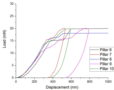
Figure 4.42- Load-displacement curves of micro-pillar indentation splitting tests and SEM front view of pillars after testing in sample HP-Al:LLZO-SG a) load-displacement curves of pillar with \sim 10 \mu\text{m} diameter; b) SEM micrographs of pillars 1 to 5 after testing; c) load-displacement curves of pillar with \sim 5 \mu\text{m} diameter; d) SEM micrographs of pillars 6 to 10 after testing.
