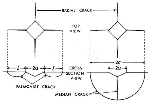
Figure 2.5- Schematic of Palmqvist cracks and median-radial cracks [114].
