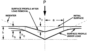
Figure 2.4- Schematic representation of a) main parameters describing the indentation process b) typical indentation load–displacement curve, where P_{\max} is the max. indentation load, h_{\max} the indenter displacement at peak load, h_f the final depth of the contact impression after unloading and S the initial unloading stiffness [105].
