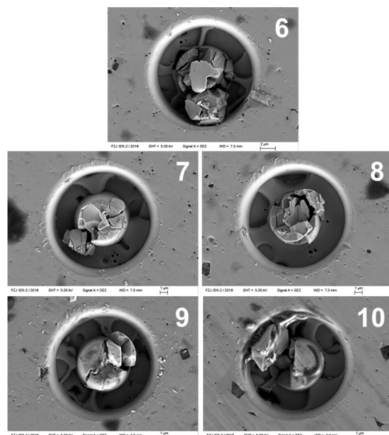
Figure 4.42- Load-displacement curves of micro-pillar indentation splitting tests and SEM front view of pillars after testing in sample HP-Al:LLZO-SG a) load-displacement curves of pillar with \sim 10 \mu\text{m} diameter; b) SEM micrographs of pillars 1 to 5 after testing; c) load-displacement curves of pillar with \sim 5 \mu\text{m} diameter; d) SEM micrographs of pillars 6 to 10 after testing.
