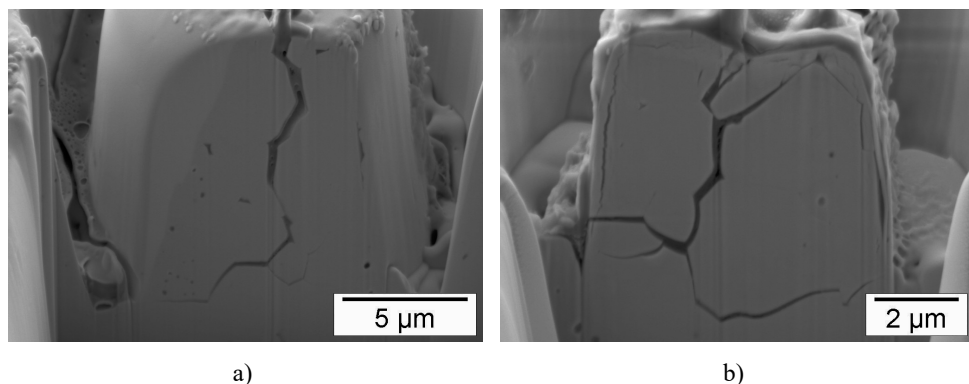
Figure 4.44 –SEM micrographs of cross-sectional FIB cut on HP-Al:LLZO-SG of a) pillar 5 (~10 \mu\text{m} diameter) b) pillar 9 (~5 \mu\text{m} diameter).
