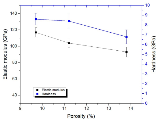
Figure 4.9 - Influence of porosity on mechanical properties of 20Al:LLZ sintered for different dwell times.
