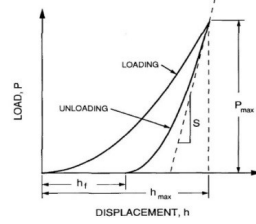
Figure 2.4- Schematic representation of a) main parameters describing the indentation process b) typical indentation load–displacement curve, where P_{\max} is the max. indentation load, h_{\max} the indenter displacement at peak load, h_f the final depth of the contact impression after unloading and S the initial unloading stiffness [105].
