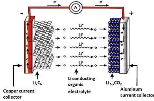
Figure 2.1- Schematic illustration of traditional lithium-ion battery [9].
