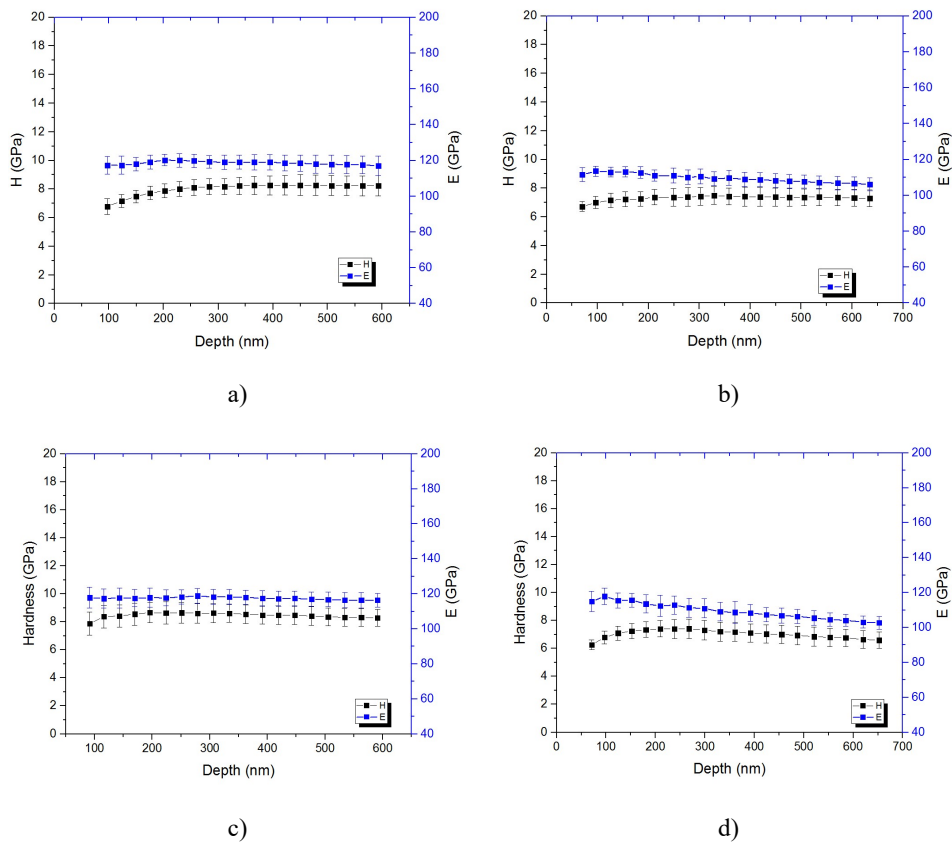
Figure 4.36 -Hardness and elastic modulus as function of penetration depth for a) HP-Al:LLZO-LG b) HP-Al:LLZO-SG c) HP-Al free:LLZO-LG d) HP-Al free:LLZO-SG.
