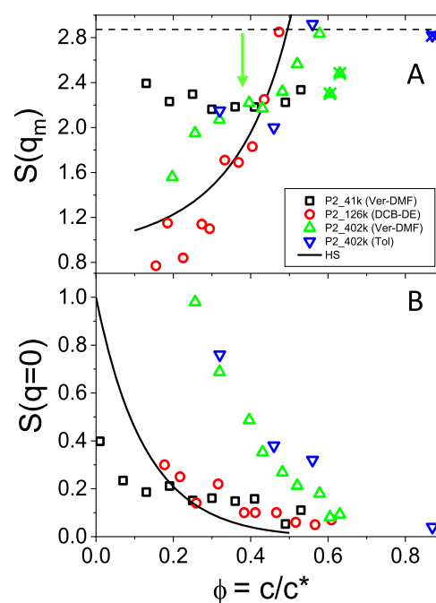
FIG. 7. (a) Structure factor principal peak height, S(q_m) , as a function of volume fraction \phi for all considered core-shell systems as indicated. The solid black curve is the hard-sphere peak height according to Eq. (16), and the horizontal dashed line indicates the Hansen-Verlet peak value 2.85 hallmarking the fluid-crystal freezing transition of hard-sphere-like systems. 39 (b) Zero- q estimated values for the osmotic compressibility factor S(0) as a function of volume fraction, for the indicated core-shell systems. The solid black line is the hard-sphere Carnahan-Starling result in Eq. (17). The depicted data (open symbols) are actually taken for the lowest attained q values.
