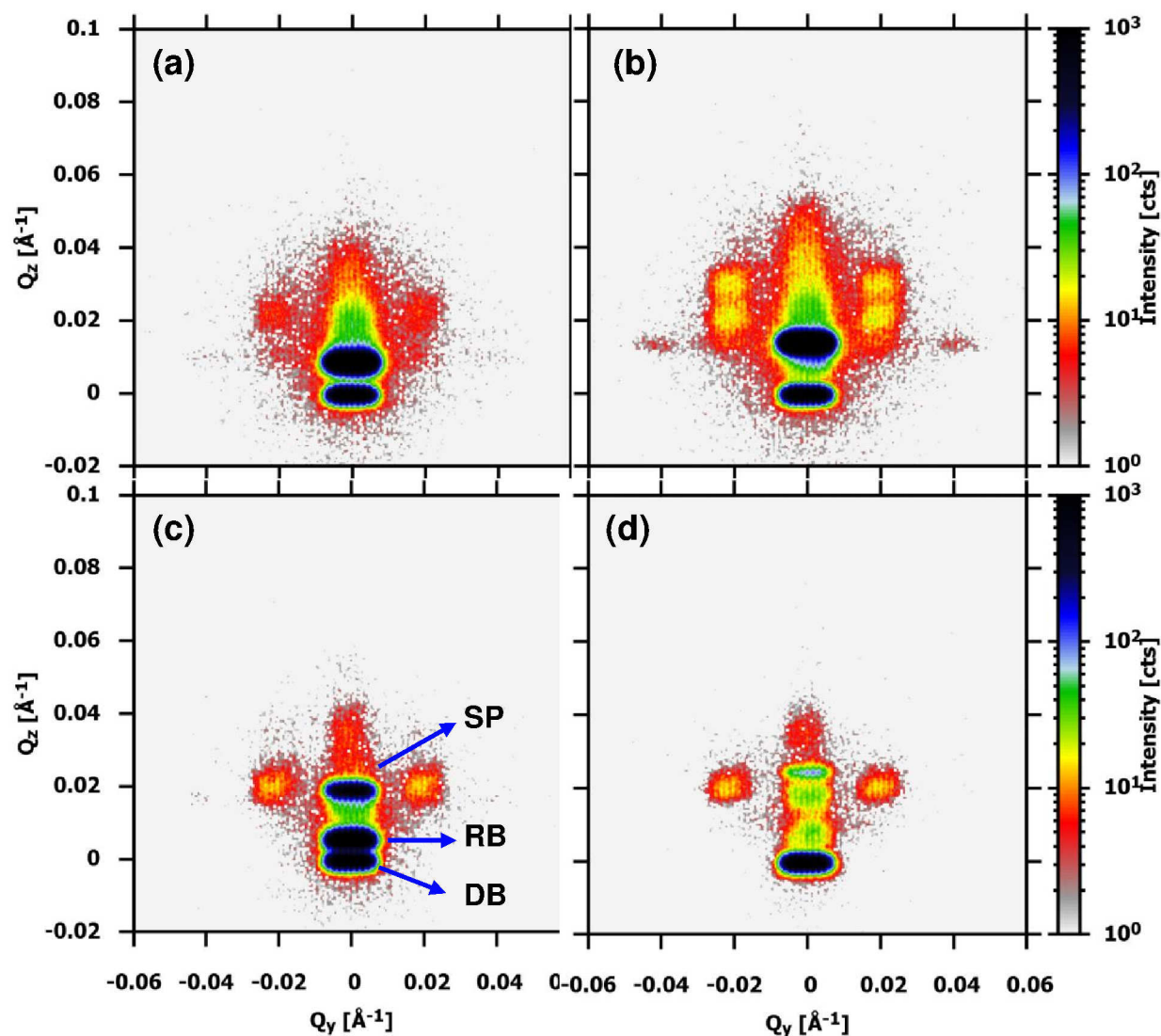
Fig. 7. 7 The GISANS data taken at incident angle of (a) 0.2^\circ (b) 0.3^\circ (c) 0.4^\circ and (d) 0.5^\circ . The specular peak (SP), refracted beam (RB) and direct beam (DB) are indicated with solid arrows.
