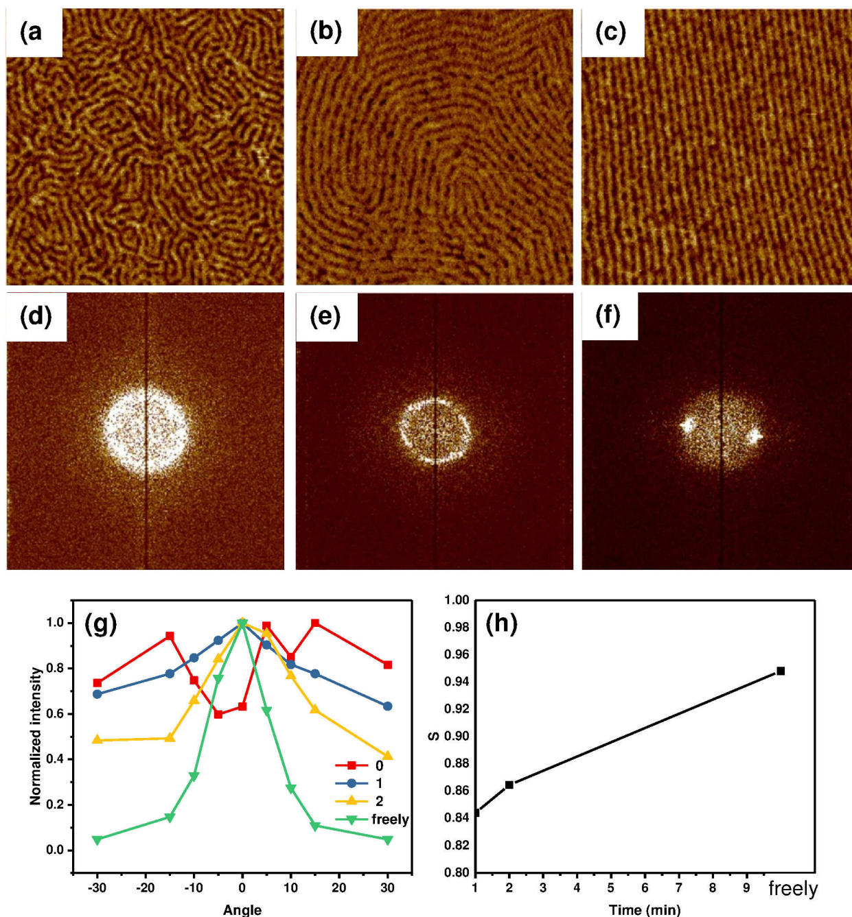
Fig. 6. 10 The AFM phase image and corresponding 2D Fourier transforms of sample resting in the jar for 0 min (a, d), 1 min (b, e) and 2 minutes (c, f) after 6 minutes solvent vapor annealing. The first order peak intensity profiles (g) and orientation parameter was obtained from the azimuthal angle dependent GISAXS.
