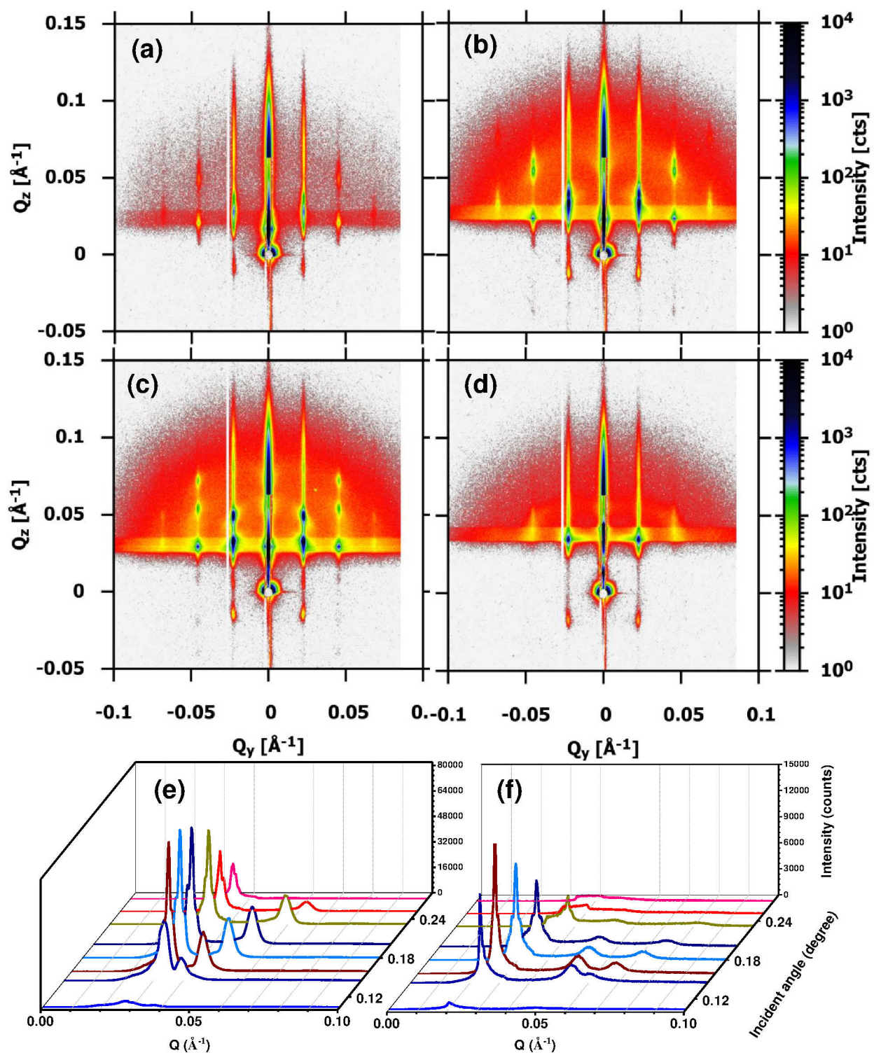
Fig. 6. 11 GISAXS measurements at different incident angles (a) 0.1 °, (b) 0.14 °, (c) 0.18 ° and (d) 0.27 °. The line cuts along Q_z direction at Q_y (e) first peak 0.0223 \text{\AA}^{-1} and (f) second peak 0.0446 \text{\AA}^{-1} .
