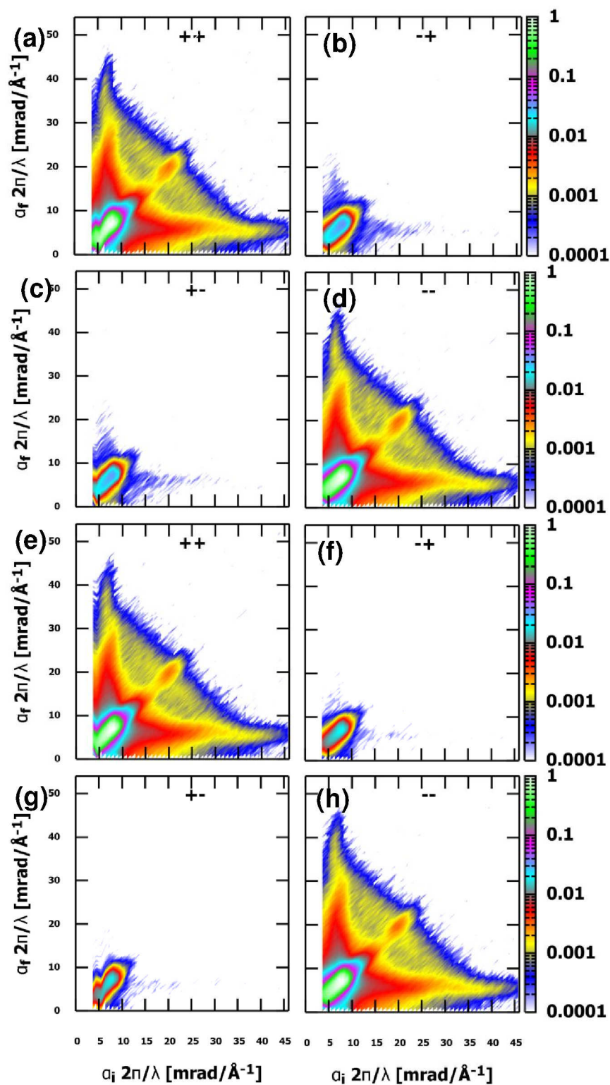
Fig. 7. 12 The off-specular map measurements taken at 5 K and at 1.1 T (a, b, c and d) and 5 mT (e, f, g and h).
