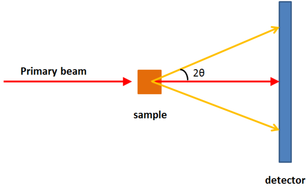
Fig. 2. 7 Small angle scattering geometry.
