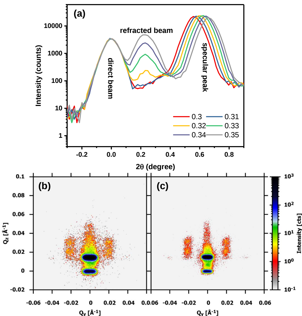
Fig. 7. 8 (a) The line cuts along specular line of GISANS at various incident angles from 0.3 to 0.35°. The GISANS measurements performed at (b) 0.31 ° with \lambda = 4.5 \text{ \AA} and (c) 0.41 ° with \lambda = 6 \text{ \AA} . All data was taken at 300 K.
