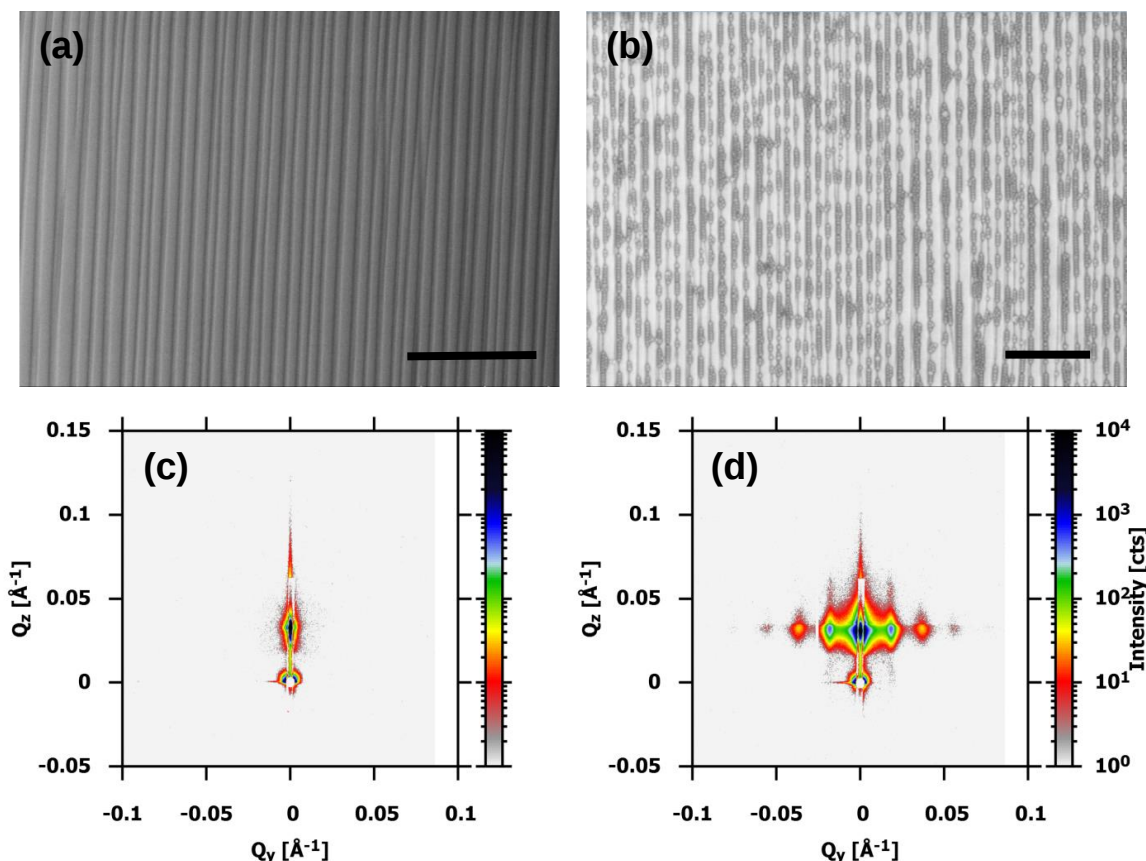
Fig. 5. 1 SEM images of (a) sap1500 and (b) sap1500-1d30 (scale bar: 1 μm). The GISAXS patterns of (c) sap1500 and (d) sap1500-1d30 with incident beam perpendicular to the ridge of patterned substrate.
