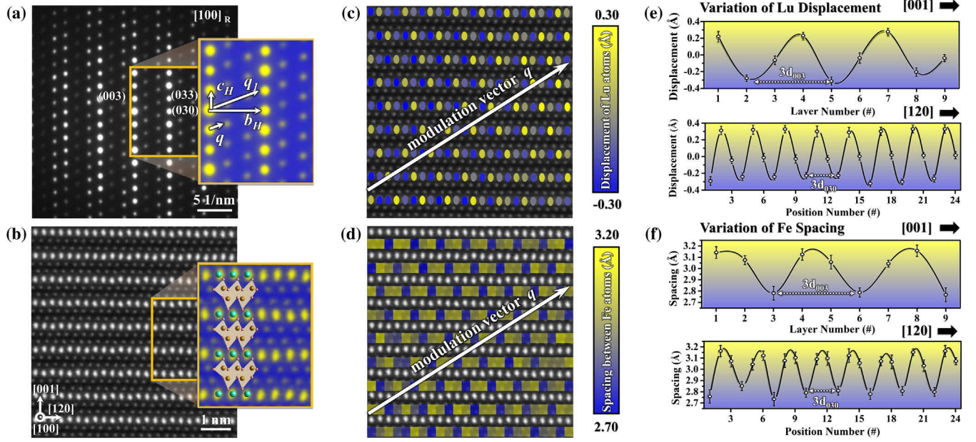
FIG. 1. Modulation structure in diffraction pattern and HAADF image. (a) Diffraction pattern along the [100] zone axis; the inset shows the relationship between the modulation vector \mathbf{q} and vector \mathbf{q}_1 . (b) HAADF image along the [100] zone axis. The enlargement highlights the [AAA] stacking sequence, consistent with the atomic model. Green, brown, and red atoms represent Lu, Fe, and O atoms, respectively. (c),(d) Maps showing the periodic variation of the Lu displacement and Fe spacing. (e),(f) Variation of the Lu displacement and the Fe spacing along the [001] and [120] directions, respectively.
