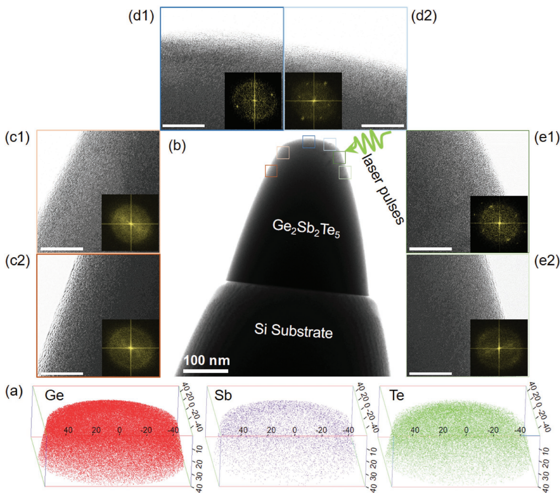
Figure 2. High-resolution correlative APT-TEM investigations showing partial laser-pulse induced crystallization of an amorphous \text{Ge}_2\text{Sb}_2\text{Te}_5 tip. a) Reconstructed 3D maps of Ge (red), Sb (blue), and Te (green) atoms obtained from APT. In total, two million ions are field evaporated from the tip by applying laser pulses. b) Bright field TEM image of the resulting tip after the APT experiment. c) Bright field high-resolution TEM images from the left-side of the tip, which show the amorphous state of GST. d,e) Bright field high-resolution TEM images from the top and right-side of the tip, respectively, which clearly show the presence of nanoscale grains in GST. The scale bar corresponds to 10 nm. The insets are the corresponding fast Fourier transformation patterns, showing these grains possess a rock-salt structure. The regions where these nanocrystallites are observed correspond exactly to those regions where the focused laser spot (beam spot size 2.5\ \mu\text{m} ) hits the specimen.
