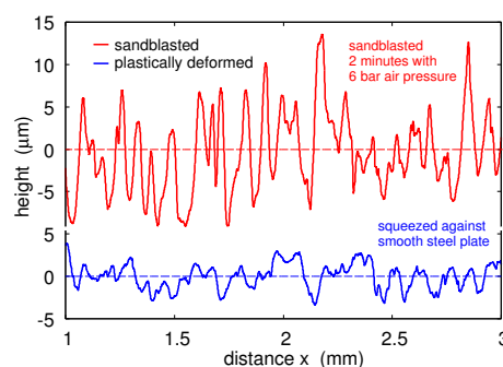
Figure 7. The surface height as a function of the distance along a straight line for the sandblasted UHMWPE sphere (red), and for the plastically deformed surface (blue) after removing the macroscopic curvature.
