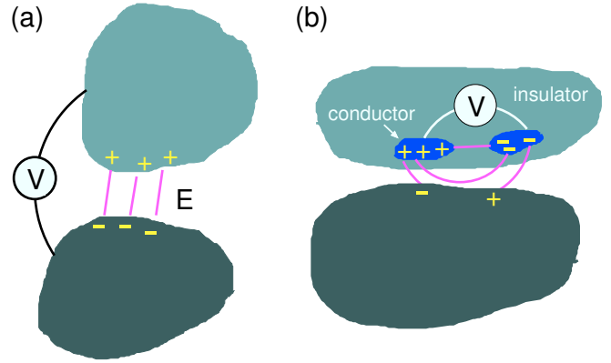
FIG. 1: An attractive electrostatic force can occur between two solid objects if (a) an electric potential difference occurs between the bodies, or if (b) an electric field occurs outside of one of the bodies due to an electric potential difference between two conductive regions inside the body.
