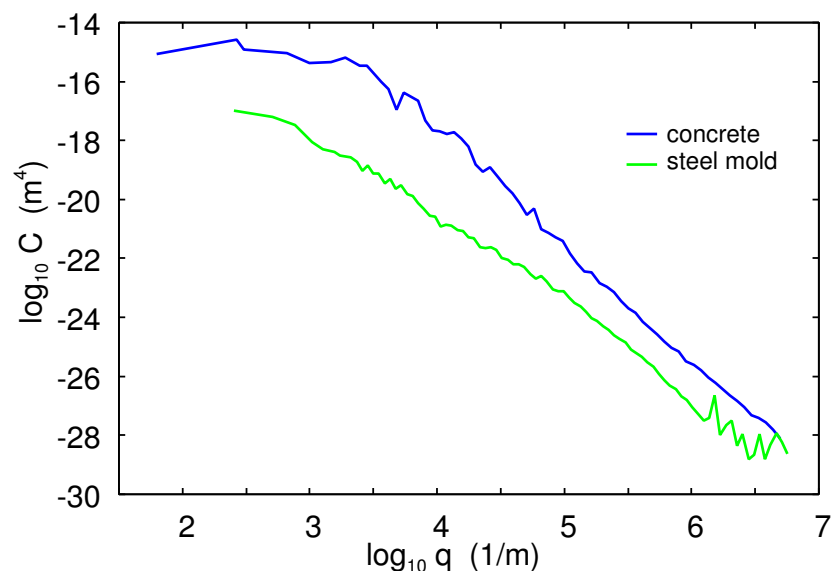
Figure 2. The 2D surface roughness power spectrum of the concrete and (rough) steel mold surfaces used in this study.
