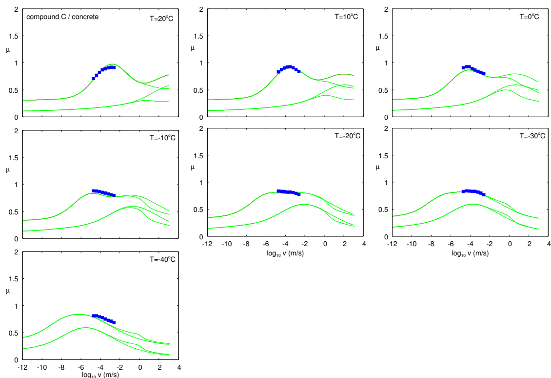
Figure 24. The friction coefficient as a function of the logarithm of sliding speed for the C rubber compound, for several temperatures. The results were from the low-temperature linear friction tester. The green lines are the theory predictions. The lower green lines are the viscoelastic contribution to the friction and the upper green lines the viscoelastic contribution plus the contribution from the area of real contact.
